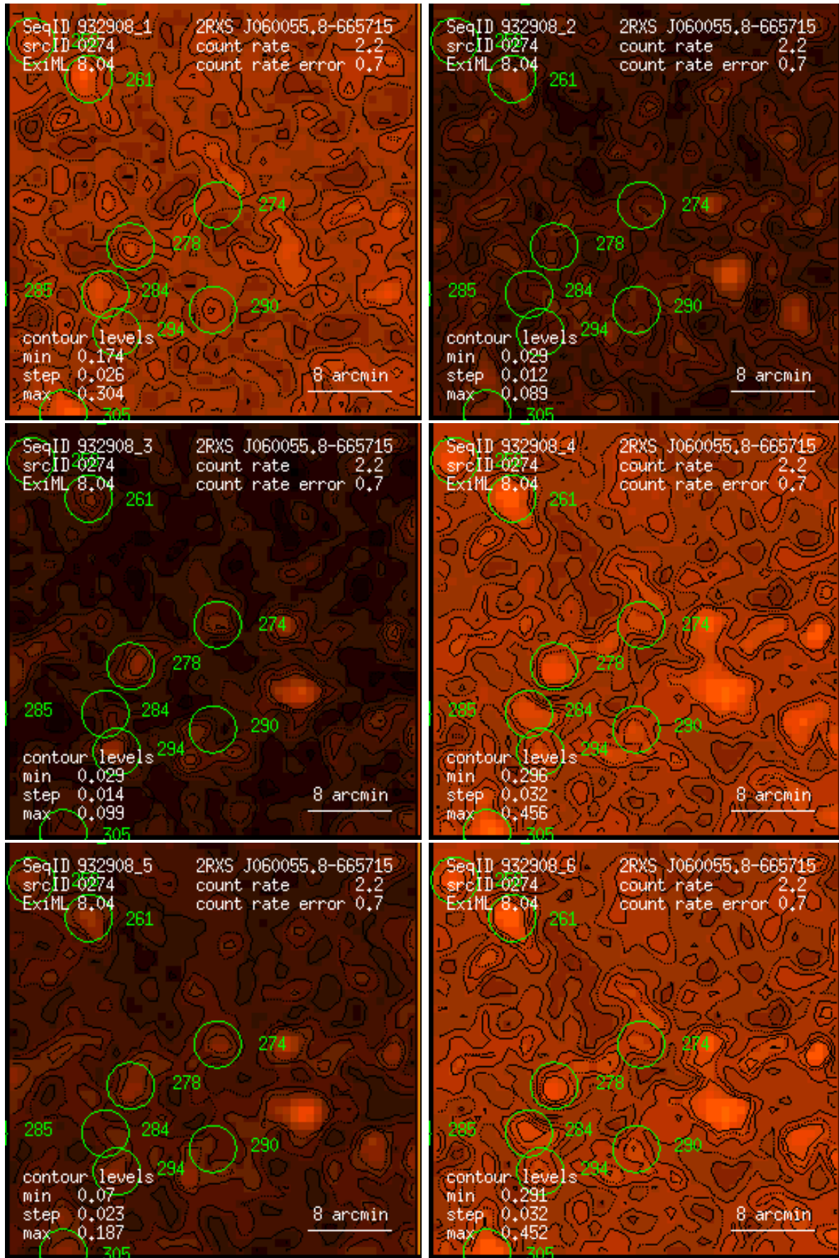
Figure 274: RASS 932908: detection 0274: band rate images, Gaussian filter: (1) PSPC channels 11 – 41, (2) 52 – 90, (3) 91 – 201, (4) 11 – 235, (5) 52 – 201, (6) 11 – 201. Broad band rates in counts/ks. Band rate contour levels in counts/ks/arcmin 2 .
