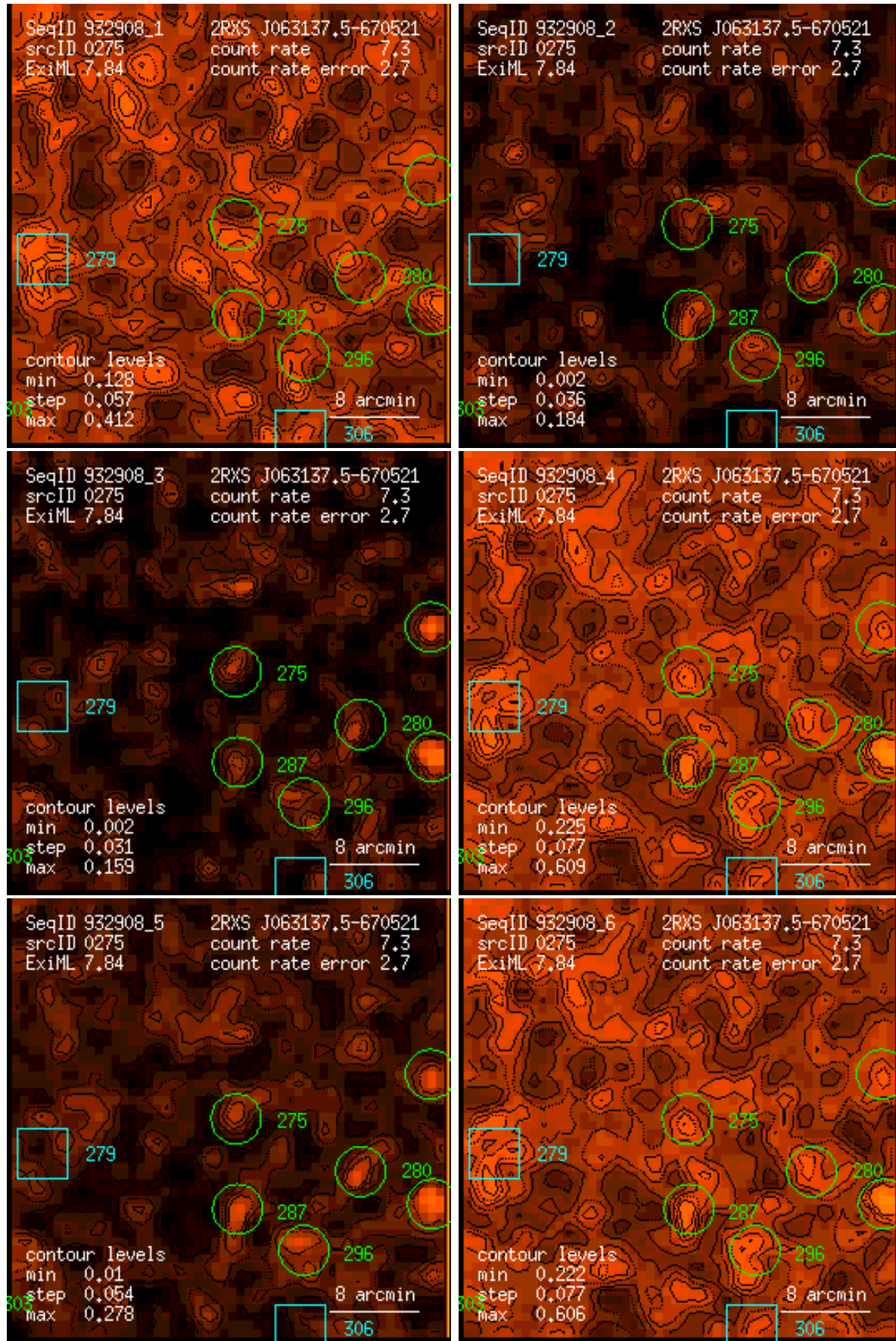
Figure 275: RASS 932908: detection 0275: band rate images, Gaussian filter: (1) PSPC channels 11 – 41, (2) 52 – 90, (3) 91 – 201, (4) 11 – 235, (5) 52 – 201, (6) 11 – 201. Broad band rates in counts/ks. Band rate contour levels in counts/ks/arcmin 2 .
