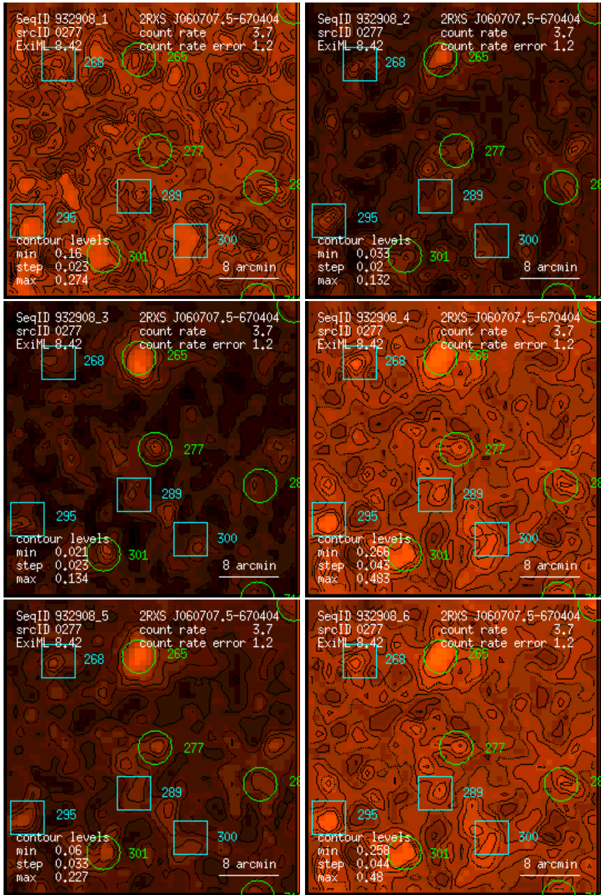
Figure 277: RASS 932908: detection 0277: band rate images, Gaussian filter: (1) PSPC channels 11 – 41, (2) 52 – 90, (3) 91 – 201, (4) 11 – 235, (5) 52 – 201, (6) 11 – 201. Broad band rates in counts/ks. Band rate contour levels in counts/ks/arcmin 2 .
