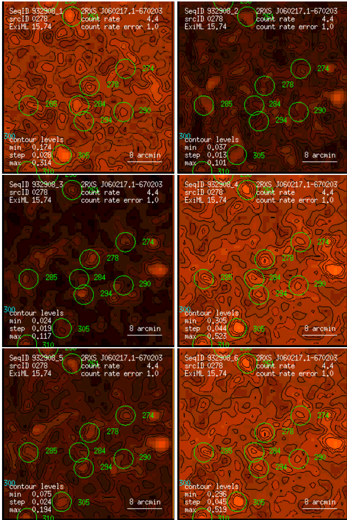
Figure 278: RASS 932908: detection 0278: band rate images, Gaussian filter: (1) PSPC channels 11 – 41, (2) 52 – 90, (3) 91 – 201, (4) 11 – 235, (5) 52 – 201, (6) 11 – 201. Broad band rates in counts/ks. Band rate contour levels in counts/ks/arcmin 2 .
