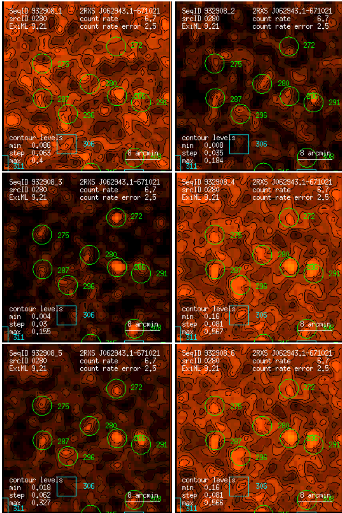
Figure 280: RASS 932908: detection 0280: band rate images, Gaussian filter: (1) PSPC channels 11 – 41, (2) 52 – 90, (3) 91 – 201, (4) 11 – 235, (5) 52 – 201, (6) 11 – 201. Broad band rates in counts/ks. Band rate contour levels in counts/ks/arcmin 2 .
