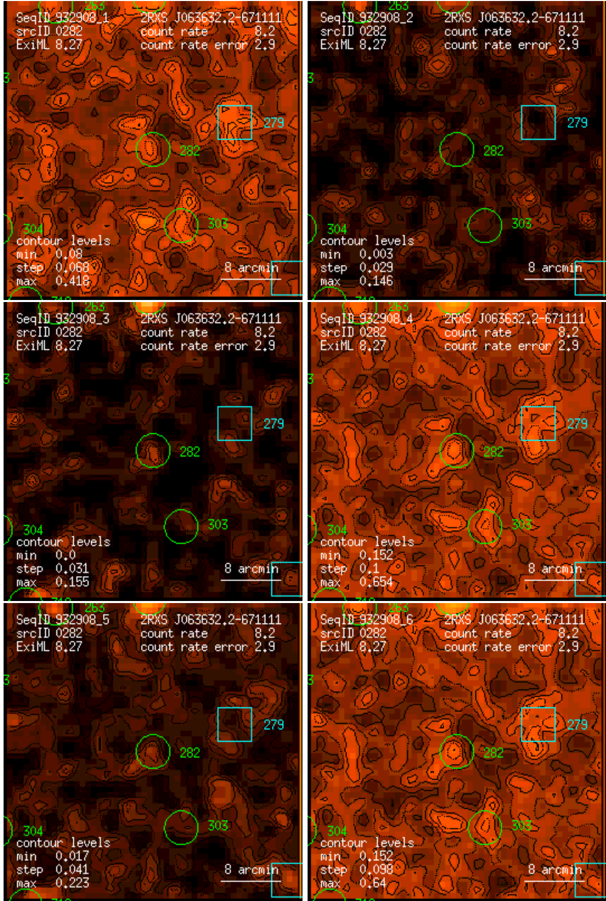
Figure 282: RASS 932908: detection 0282: band rate images, Gaussian filter: (1) PSPC channels 11 – 41, (2) 52 – 90, (3) 91 – 201, (4) 11 – 235, (5) 52 – 201, (6) 11 – 201. Broad band rates in counts/ks. Band rate contour levels in counts/ks/arcmin 2 .
