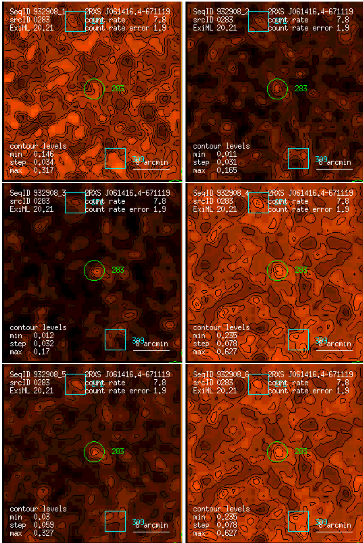
Figure 283: RASS 932908: detection 0283: band rate images, Gaussian filter: (1) PSPC channels 11 – 41, (2) 52 – 90, (3) 91 – 201, (4) 11 – 235, (5) 52 – 201, (6) 11 – 201. Broad band rates in counts/ks. Band rate contour levels in counts/ks/arcmin 2 .
