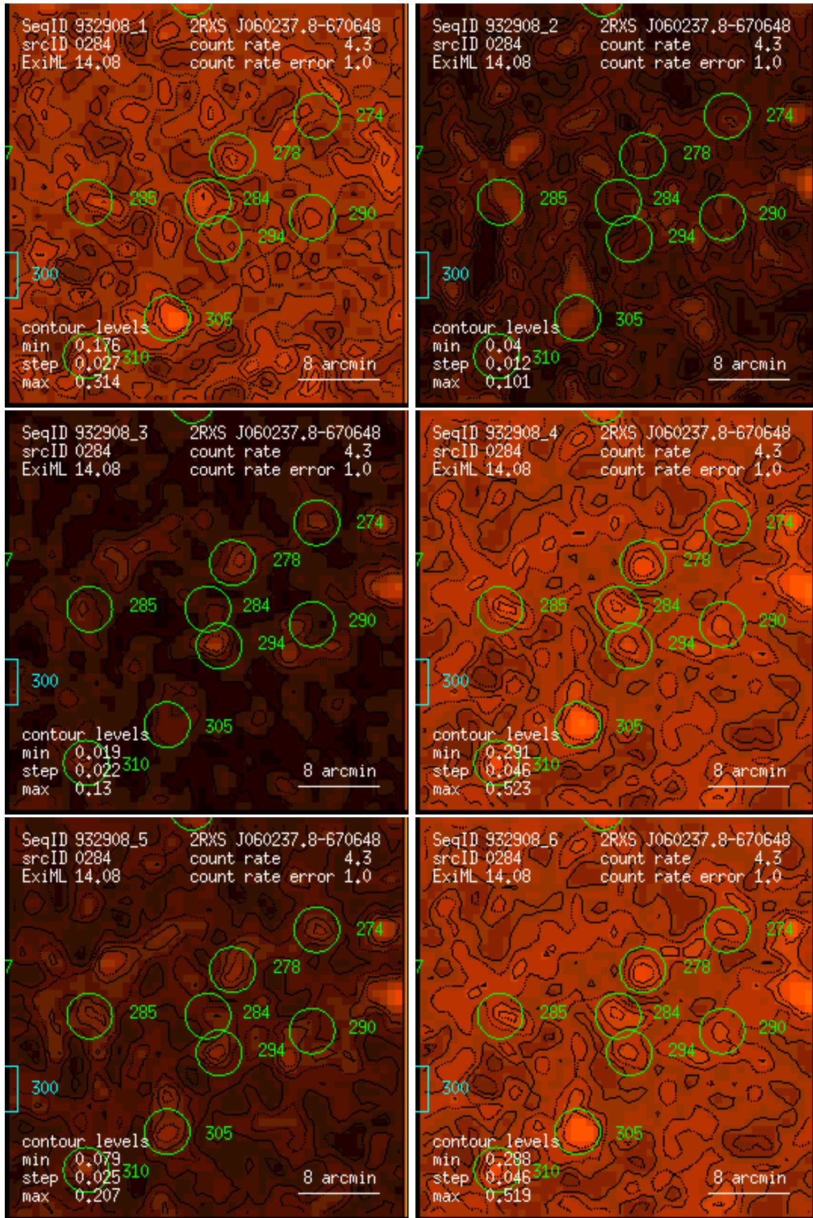
Figure 284: RASS 932908: detection 0284: band rate images, Gaussian filter: (1) PSPC channels 11 – 41, (2) 52 – 90, (3) 91 – 201, (4) 11 – 235, (5) 52 – 201, (6) 11 – 201. Broad band rates in counts/ks. Band rate contour levels in counts/ks/arcmin 2 .
