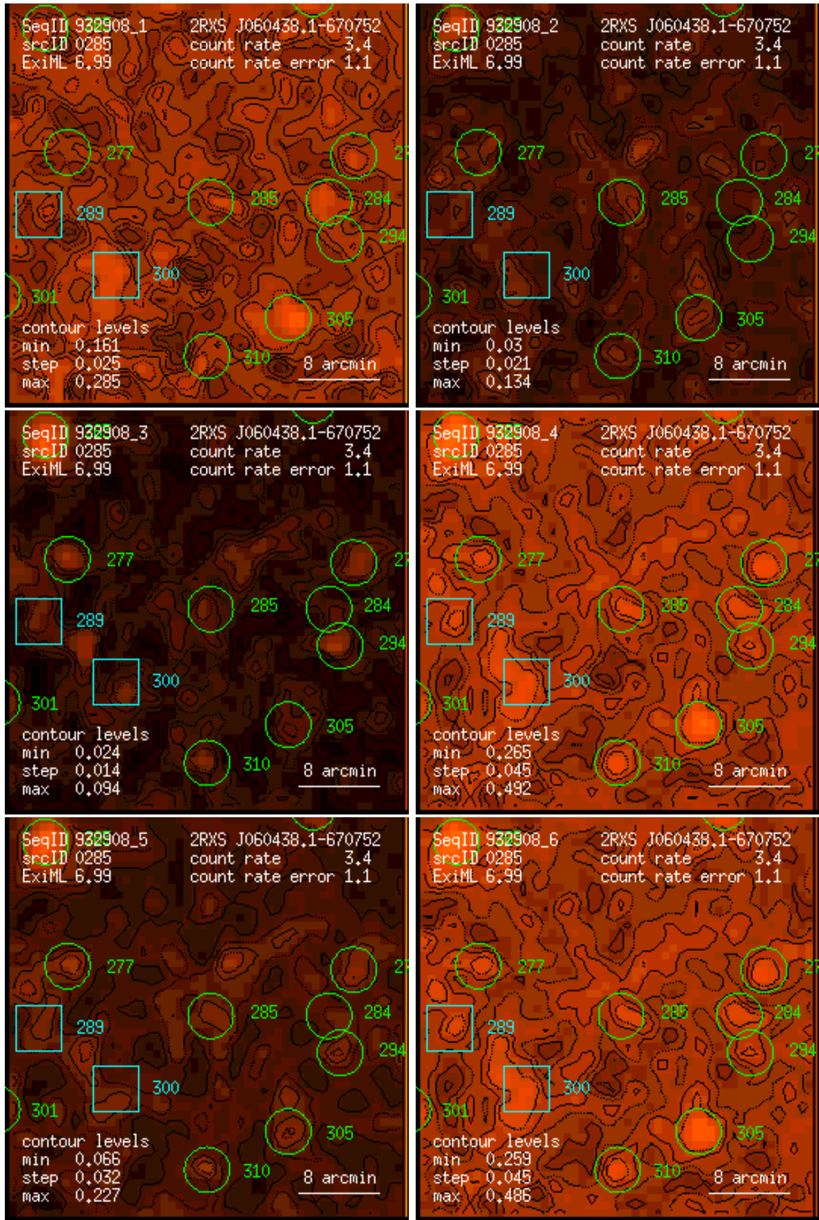
Figure 285: RASS 932908: detection 0285: band rate images, Gaussian filter: (1) PSPC channels 11 – 41, (2) 52 – 90, (3) 91 – 201, (4) 11 – 235, (5) 52 – 201, (6) 11 – 201. Broad band rates in counts/ks. Band rate contour levels in counts/ks/arcmin 2 .
