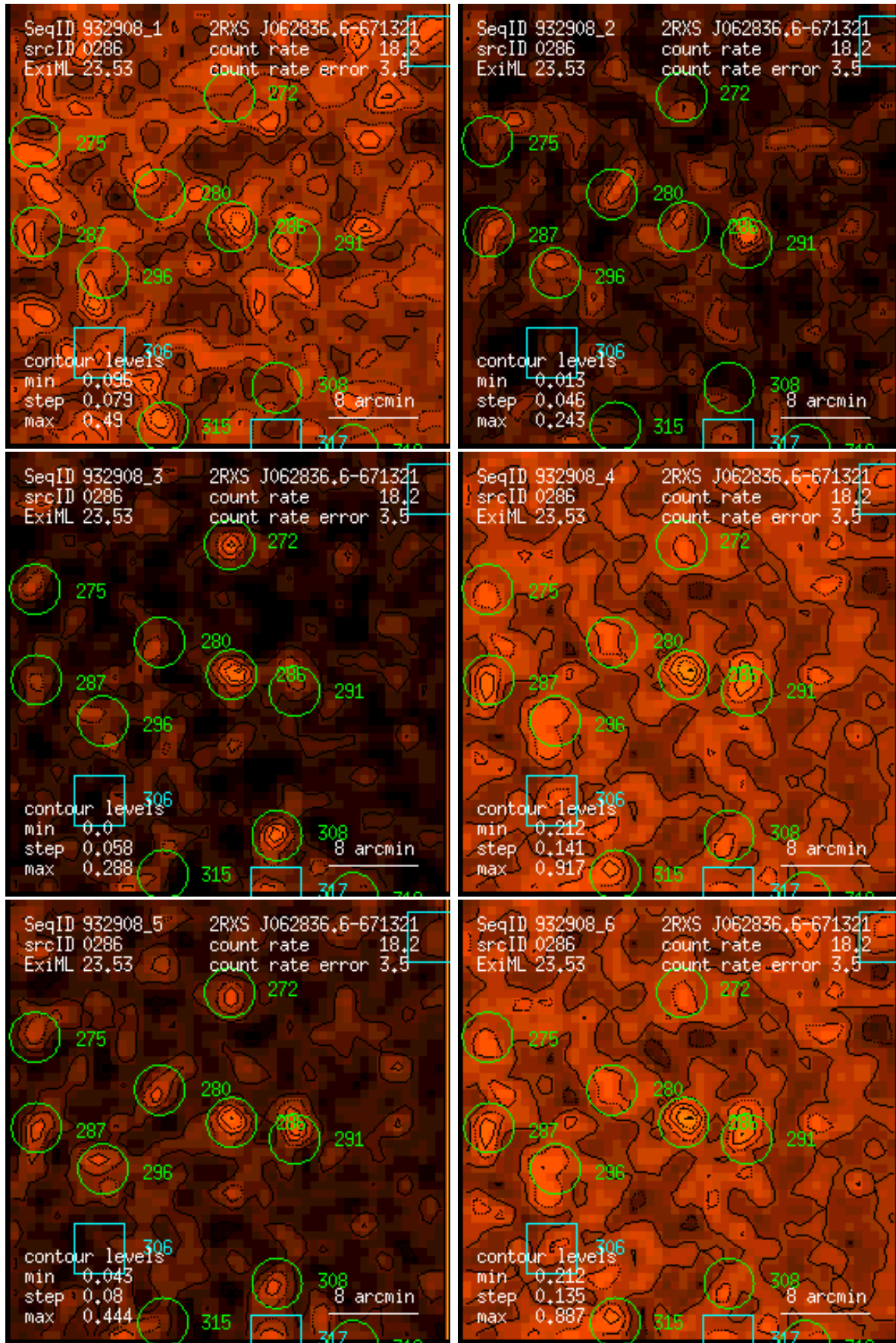
Figure 286: RASS 932908: detection 0286: band rate images, Gaussian filter: (1) PSPC channels 11 – 41, (2) 52 – 90, (3) 91 – 201, (4) 11 – 235, (5) 52 – 201, (6) 11 – 201. Broad band rates in counts/ks. Band rate contour levels in counts/ks/arcmin 2 .
