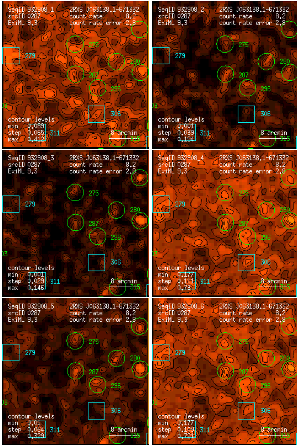
Figure 287: RASS 932908: detection 0287: band rate images, Gaussian filter: (1) PSPC channels 11 – 41, (2) 52 – 90, (3) 91 – 201, (4) 11 – 235, (5) 52 – 201, (6) 11 – 201. Broad band rates in counts/ks. Band rate contour levels in counts/ks/arcmin 2 .
