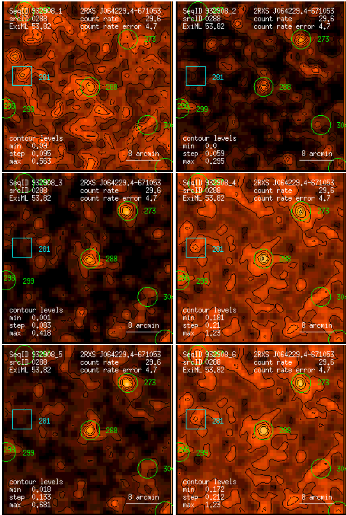
Figure 288: RASS 932908: detection 0288: band rate images, Gaussian filter: (1) PSPC channels 11 – 41, (2) 52 – 90, (3) 91 – 201, (4) 11 – 235, (5) 52 – 201, (6) 11 – 201. Broad band rates in counts/ks. Band rate contour levels in counts/ks/arcmin 2 .
