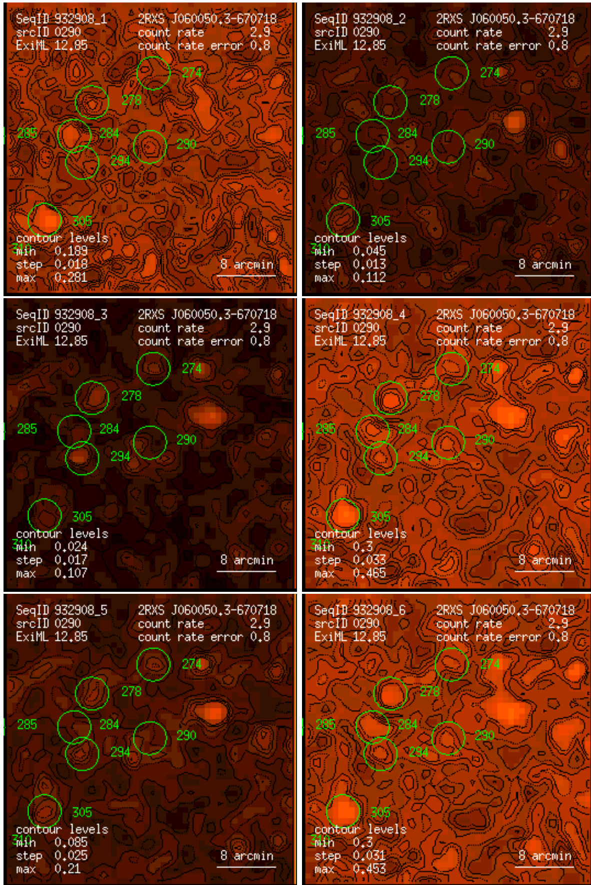
Figure 290: RASS 932908: detection 0290: band rate images, Gaussian filter: (1) PSPC channels 11 – 41, (2) 52 – 90, (3) 91 – 201, (4) 11 – 235, (5) 52 – 201, (6) 11 – 201. Broad band rates in counts/ks. Band rate contour levels in counts/ks/arcmin 2 .
