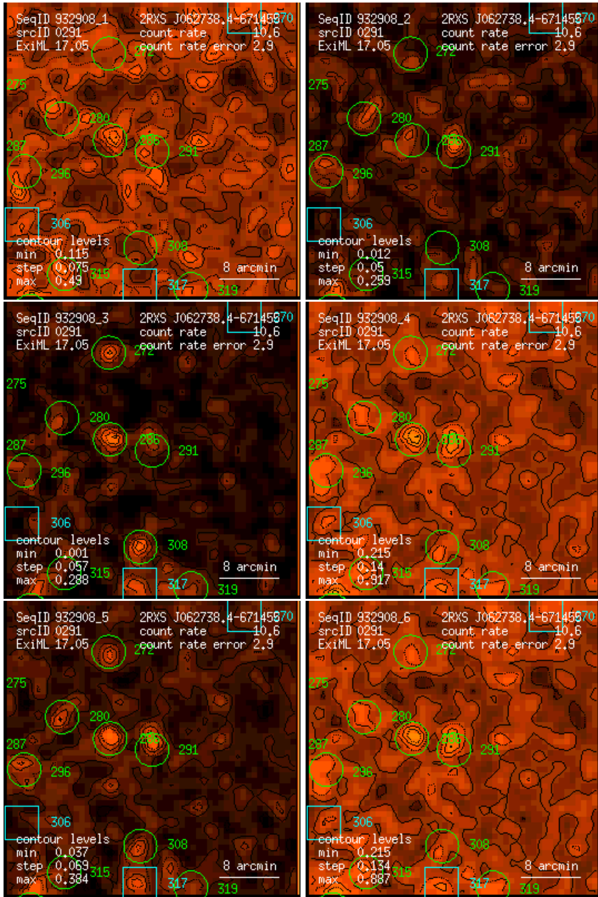
Figure 291: RASS 932908: detection 0291: band rate images, Gaussian filter: (1) PSPC channels 11 – 41, (2) 52 – 90, (3) 91 – 201, (4) 11 – 235, (5) 52 – 201, (6) 11 – 201. Broad band rates in counts/ks. Band rate contour levels in counts/ks/arcmin 2 .
