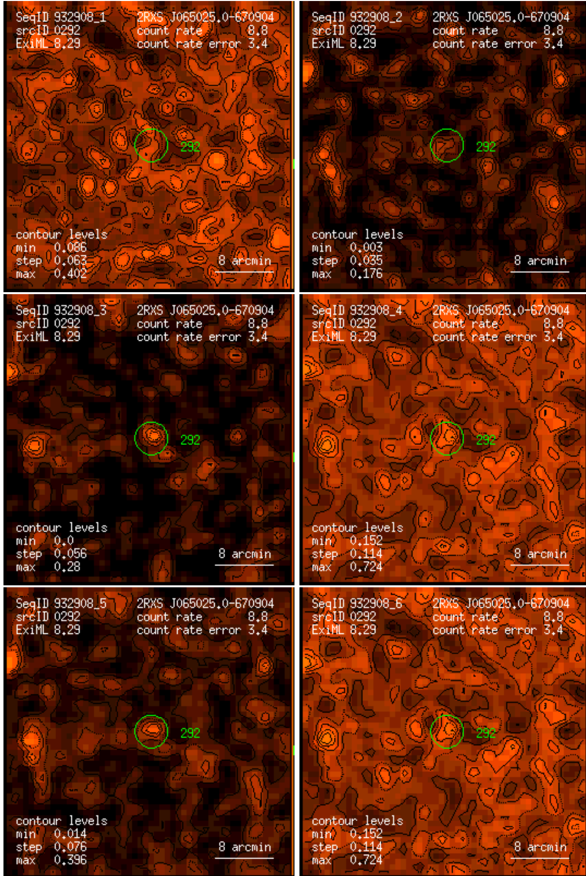
Figure 292: RASS 932908: detection 0292: band rate images, Gaussian filter: (1) PSPC channels 11 – 41, (2) 52 – 90, (3) 91 – 201, (4) 11 – 235, (5) 52 – 201, (6) 11 – 201. Broad band rates in counts/ks. Band rate contour levels in counts/ks/arcmin 2 .
