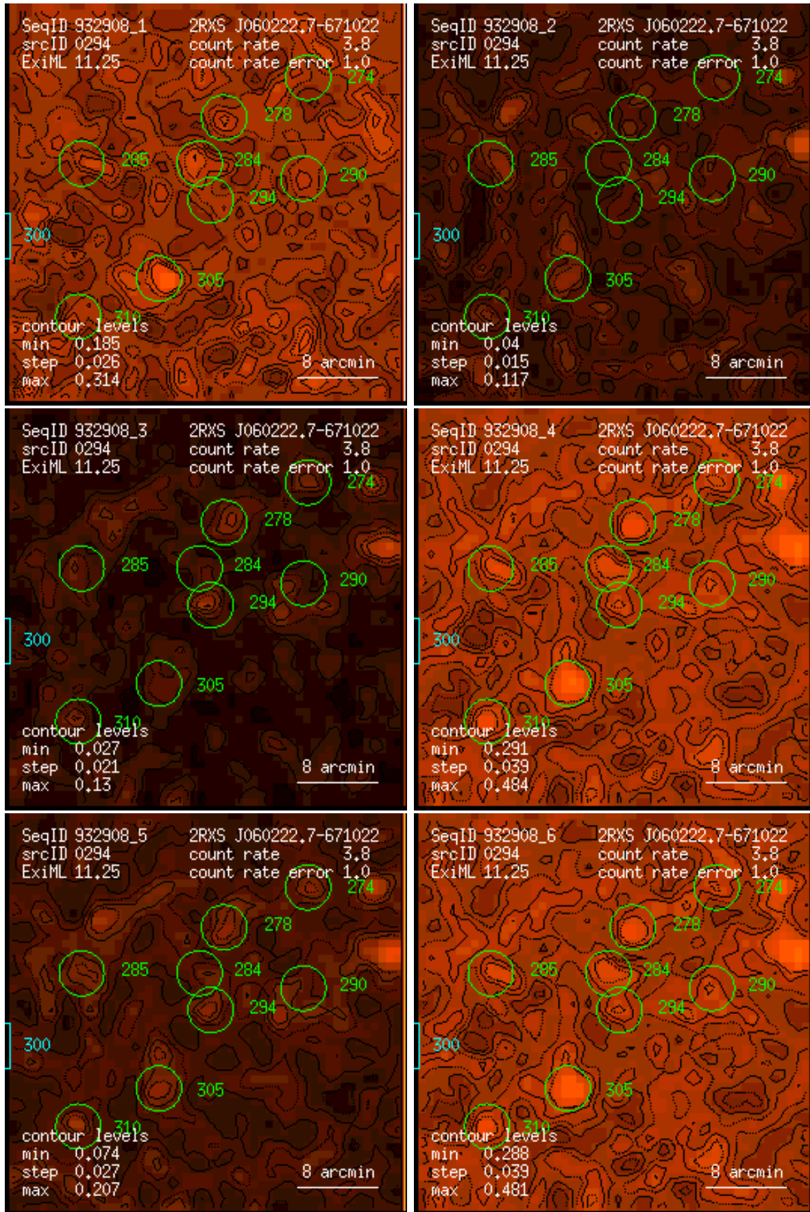
Figure 294: RASS 932908: detection 0294: band rate images, Gaussian filter: (1) PSPC channels 11 – 41, (2) 52 – 90, (3) 91 – 201, (4) 11 – 235, (5) 52 – 201, (6) 11 – 201. Broad band rates in counts/ks. Band rate contour levels in counts/ks/arcmin 2 .
