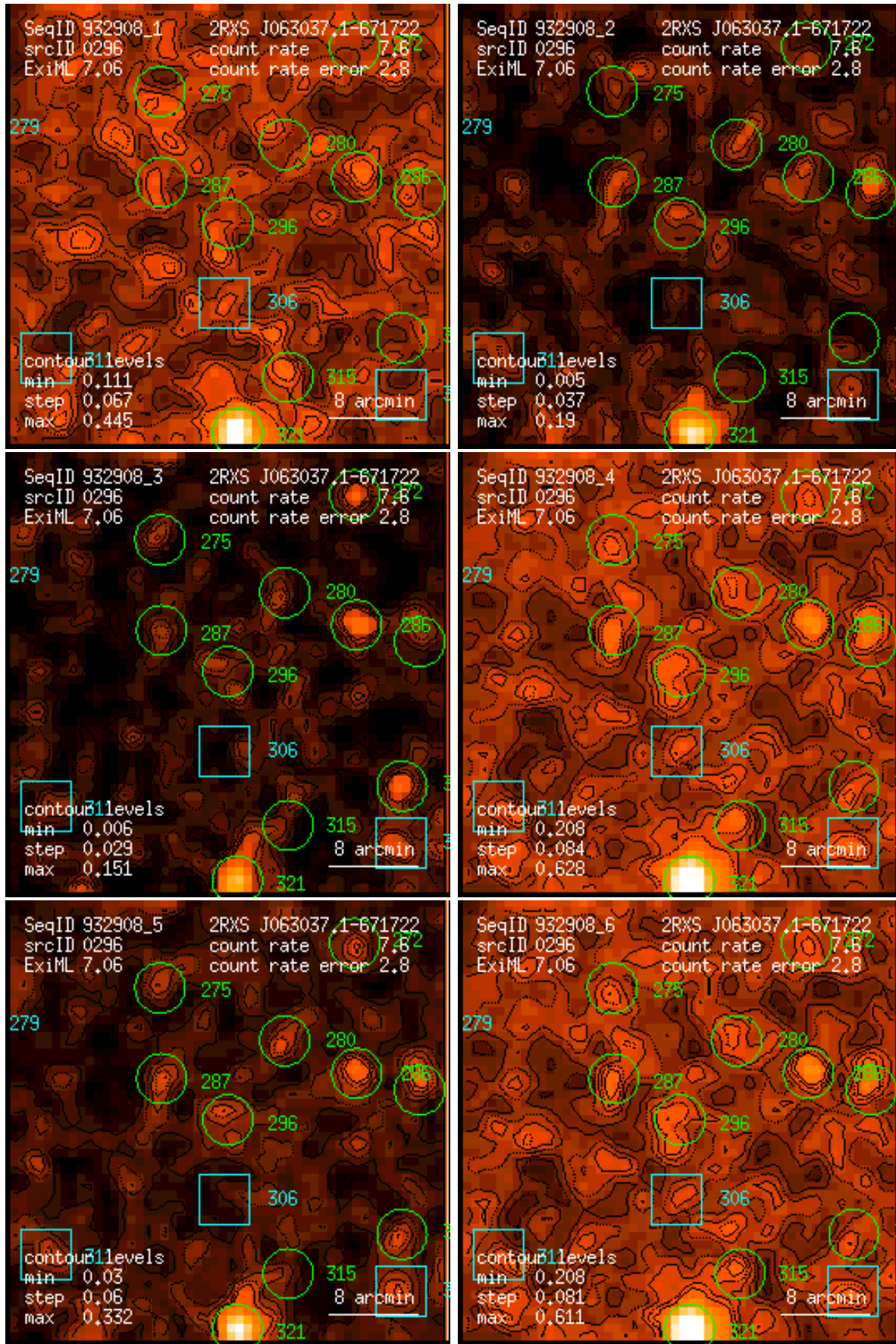
Figure 296: RASS 932908: detection 0296: band rate images, Gaussian filter: (1) PSPC channels 11 – 41, (2) 52 – 90, (3) 91 – 201, (4) 11 – 235, (5) 52 – 201, (6) 11 – 201. Broad band rates in counts/ks. Band rate contour levels in counts/ks/arcmin 2 .
