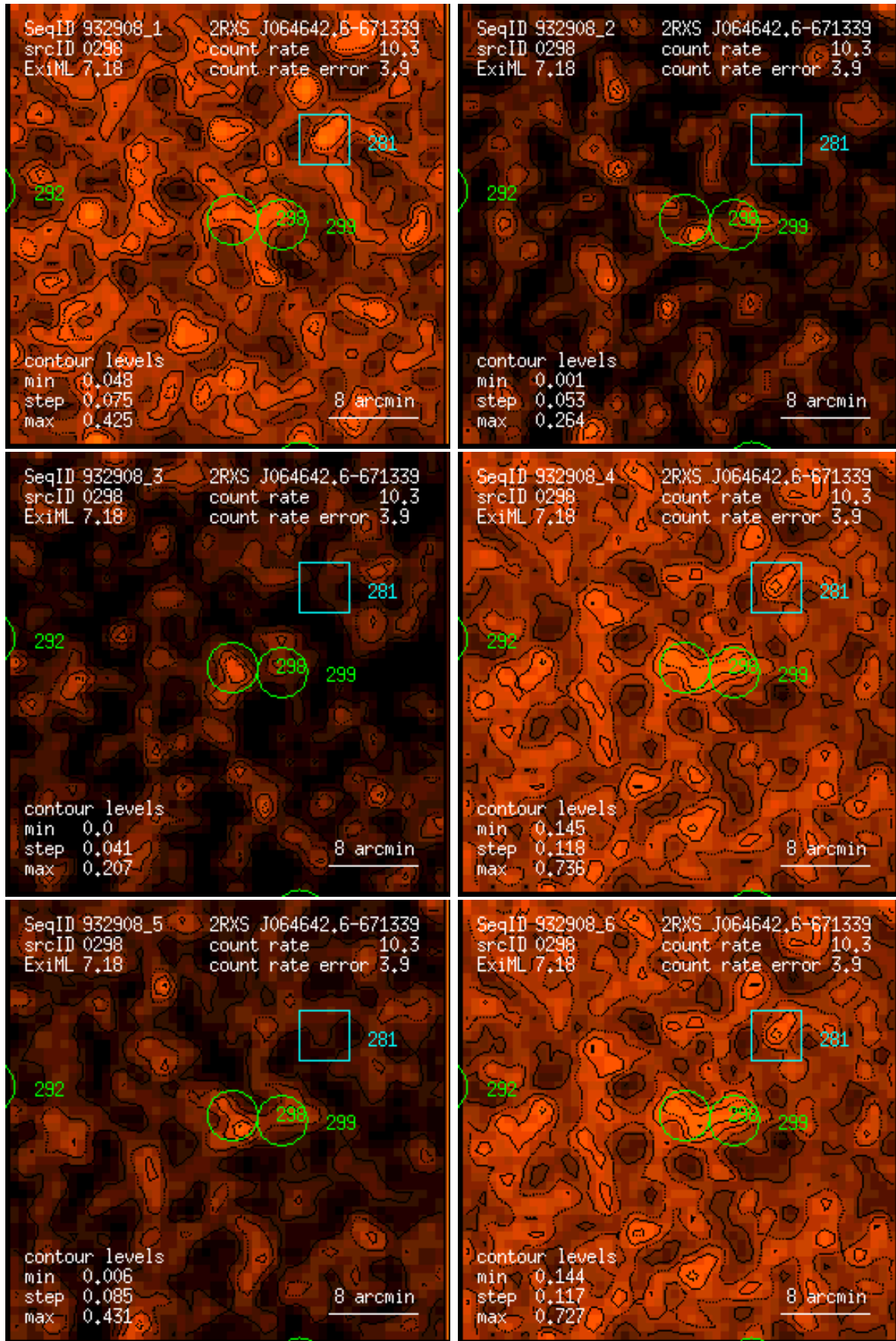
Figure 298: RASS 932908: detection 0298: band rate images, Gaussian filter: (1) PSPC channels 11 – 41, (2) 52 – 90, (3) 91 – 201, (4) 11 – 235, (5) 52 – 201, (6) 11 – 201. Broad band rates in counts/ks. Band rate contour levels in counts/ks/arcmin 2 .
