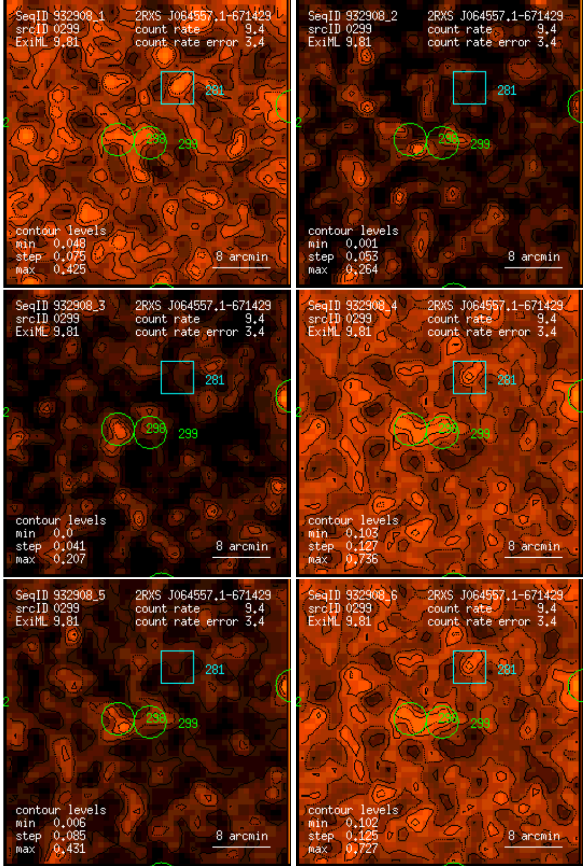
Figure 299: RASS 932908: detection 0299: band rate images, Gaussian filter: (1) PSPC channels 11 – 41, (2) 52 – 90, (3) 91 – 201, (4) 11 – 235, (5) 52 – 201, (6) 11 – 201. Broad band rates in counts/ks. Band rate contour levels in counts/ks/arcmin 2 .
