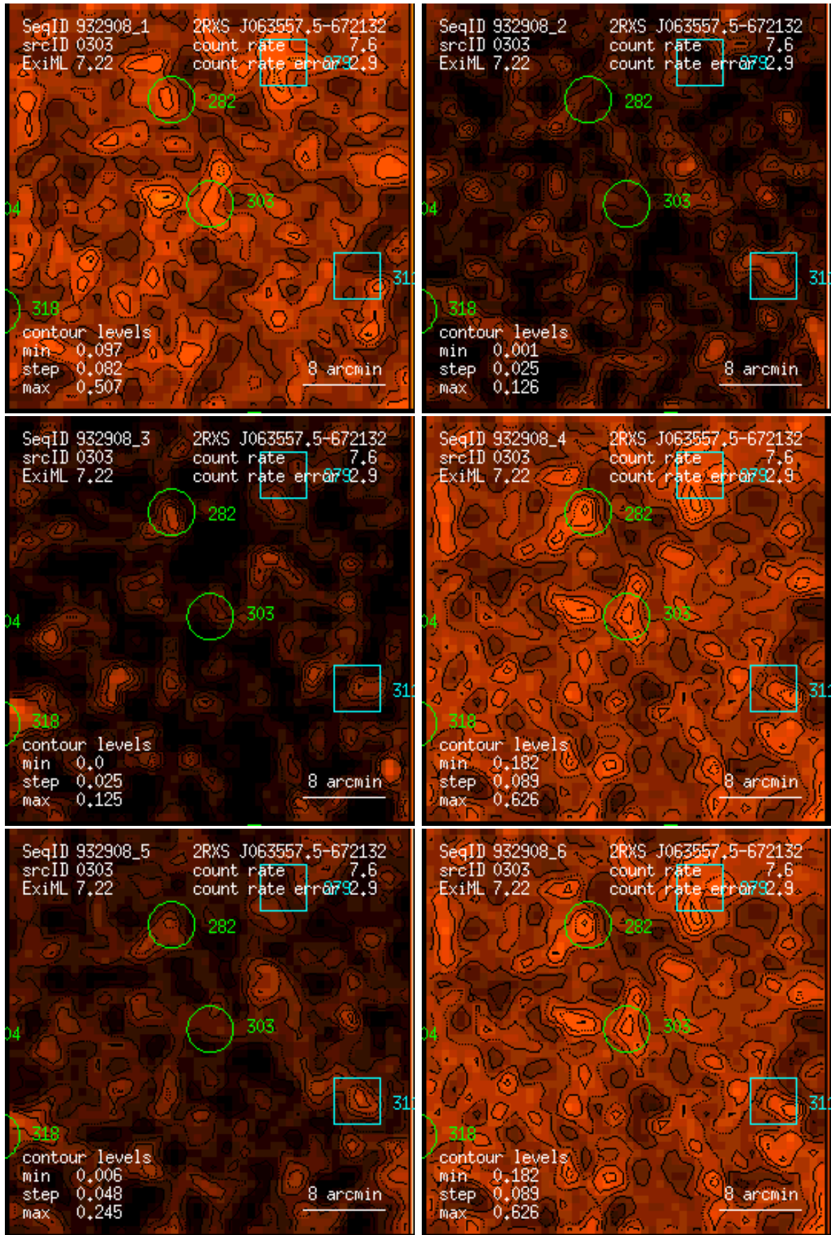
Figure 303: RASS 932908: detection 0303: band rate images, Gaussian filter: (1) PSPC channels 11 – 41, (2) 52 – 90, (3) 91 – 201, (4) 11 – 235, (5) 52 – 201, (6) 11 – 201. Broad band rates in counts/ks. Band rate contour levels in counts/ks/arcmin 2 .
