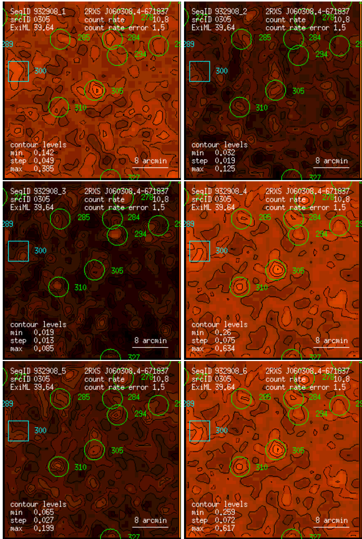
Figure 305: RASS 932908: detection 0305: band rate images, Gaussian filter: (1) PSPC channels 11 – 41, (2) 52 – 90, (3) 91 – 201, (4) 11 – 235, (5) 52 – 201, (6) 11 – 201. Broad band rates in counts/ks. Band rate contour levels in counts/ks/arcmin 2 .
