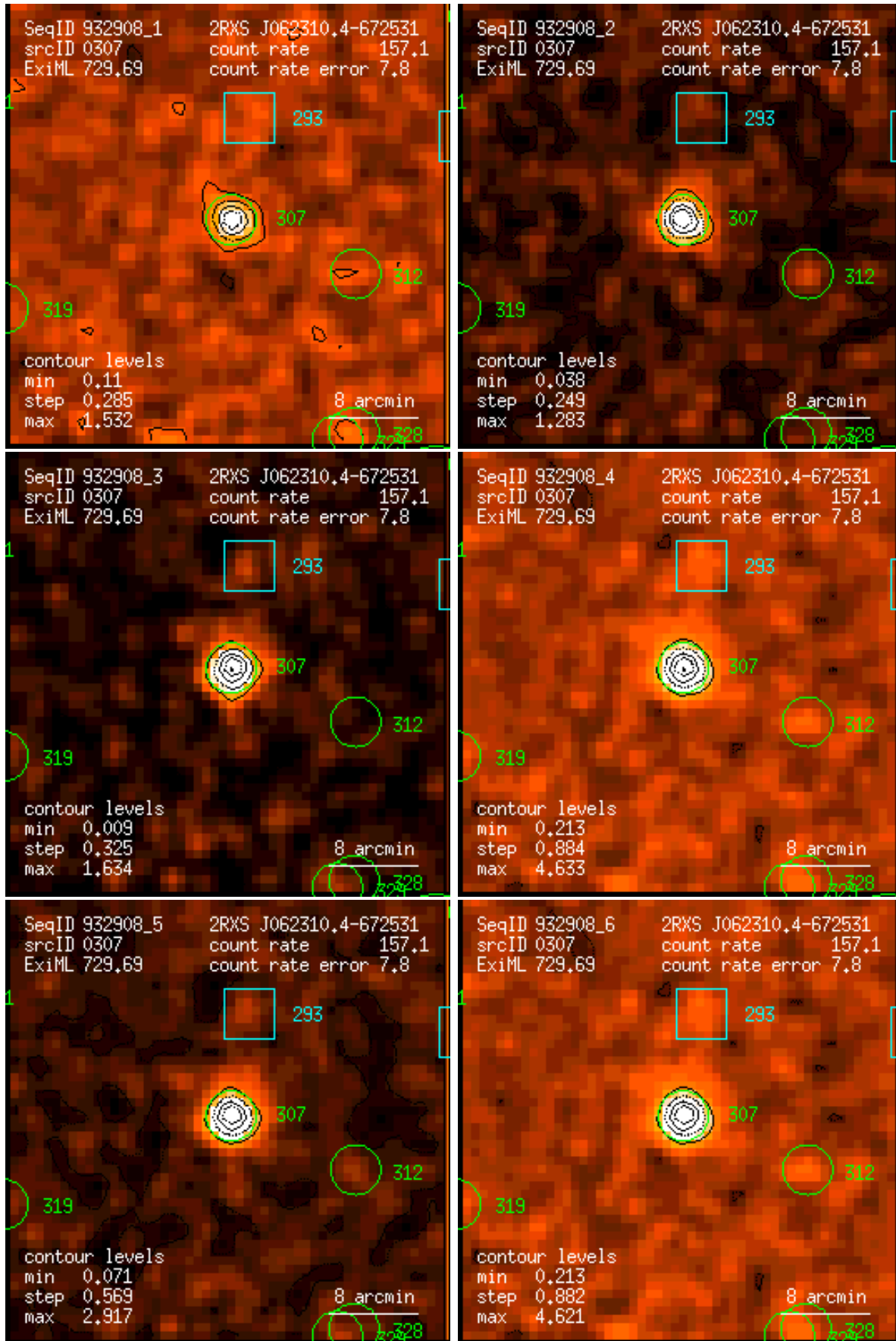
Figure 307: RASS 932908: detection 0307: band rate images, Gaussian filter: (1) PSPC channels 11 – 41, (2) 52 – 90, (3) 91 – 201, (4) 11 – 235, (5) 52 – 201, (6) 11 – 201. Broad band rates in counts/ks. Band rate contour levels in counts/ks/arcmin 2 .
