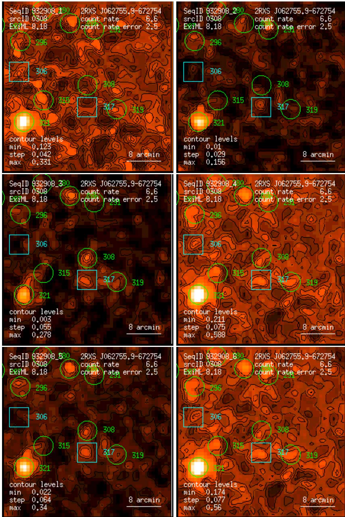
Figure 308: RASS 932908: detection 0308: band rate images, Gaussian filter: (1) PSPC channels 11 – 41, (2) 52 – 90, (3) 91 – 201, (4) 11 – 235, (5) 52 – 201, (6) 11 – 201. Broad band rates in counts/ks. Band rate contour levels in counts/ks/arcmin 2 .
