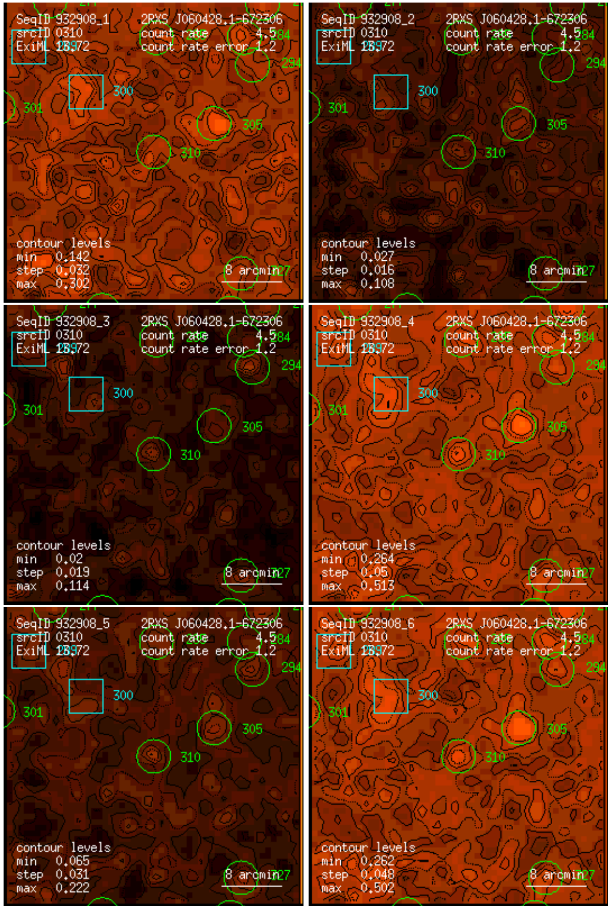
Figure 310: RASS 932908: detection 0310: band rate images, Gaussian filter: (1) PSPC channels 11 – 41, (2) 52 – 90, (3) 91 – 201, (4) 11 – 235, (5) 52 – 201, (6) 11 – 201. Broad band rates in counts/ks. Band rate contour levels in counts/ks/arcmin 2 .
