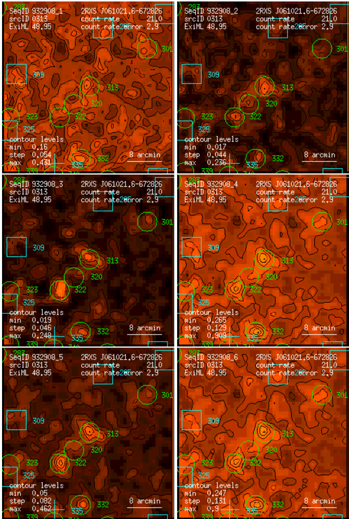
Figure 313: RASS 932908: detection 0313: band rate images, Gaussian filter: (1) PSPC channels 11 – 41, (2) 52 – 90, (3) 91 – 201, (4) 11 – 235, (5) 52 – 201, (6) 11 – 201. Broad band rates in counts/ks. Band rate contour levels in counts/ks/arcmin 2 .
