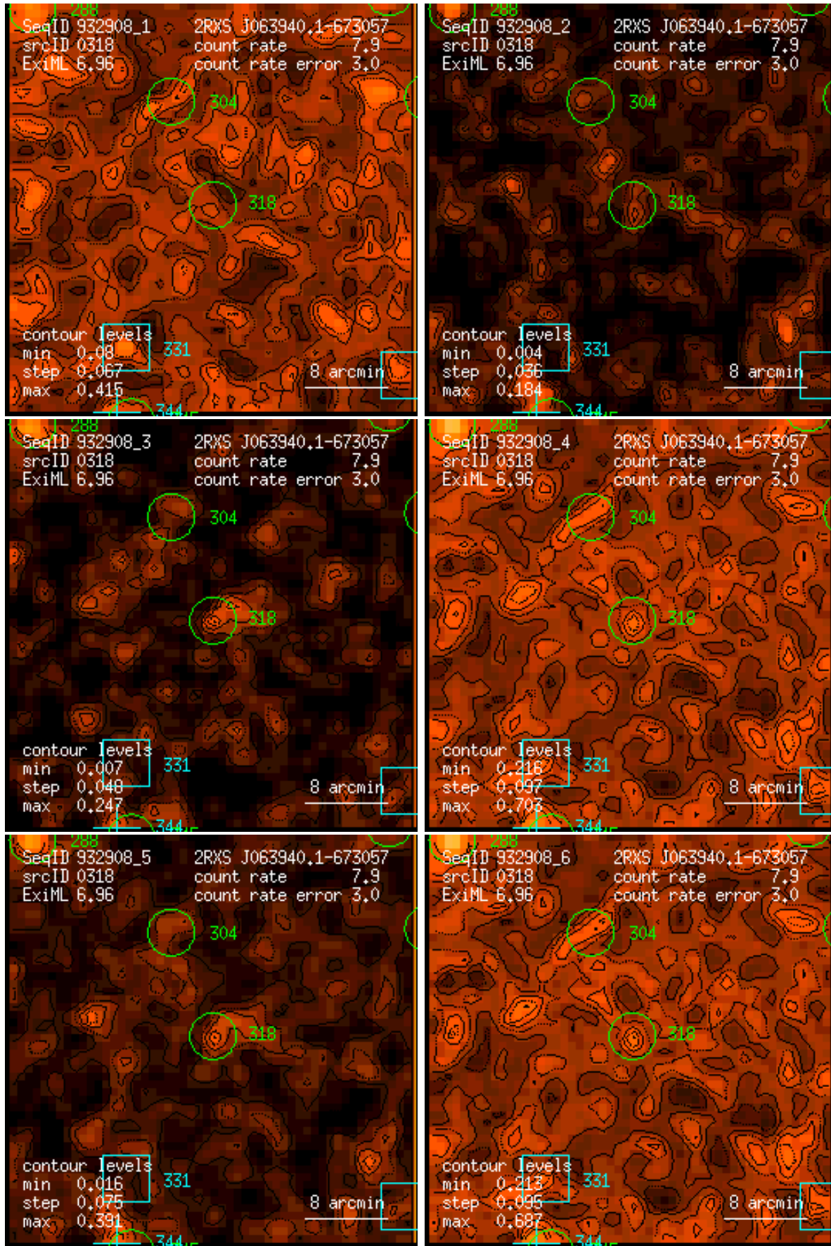
Figure 318: RASS 932908: detection 0318: band rate images, Gaussian filter: (1) PSPC channels 11 – 41, (2) 52 – 90, (3) 91 – 201, (4) 11 – 235, (5) 52 – 201, (6) 11 – 201. Broad band rates in counts/ks. Band rate contour levels in counts/ks/arcmin 2 .
