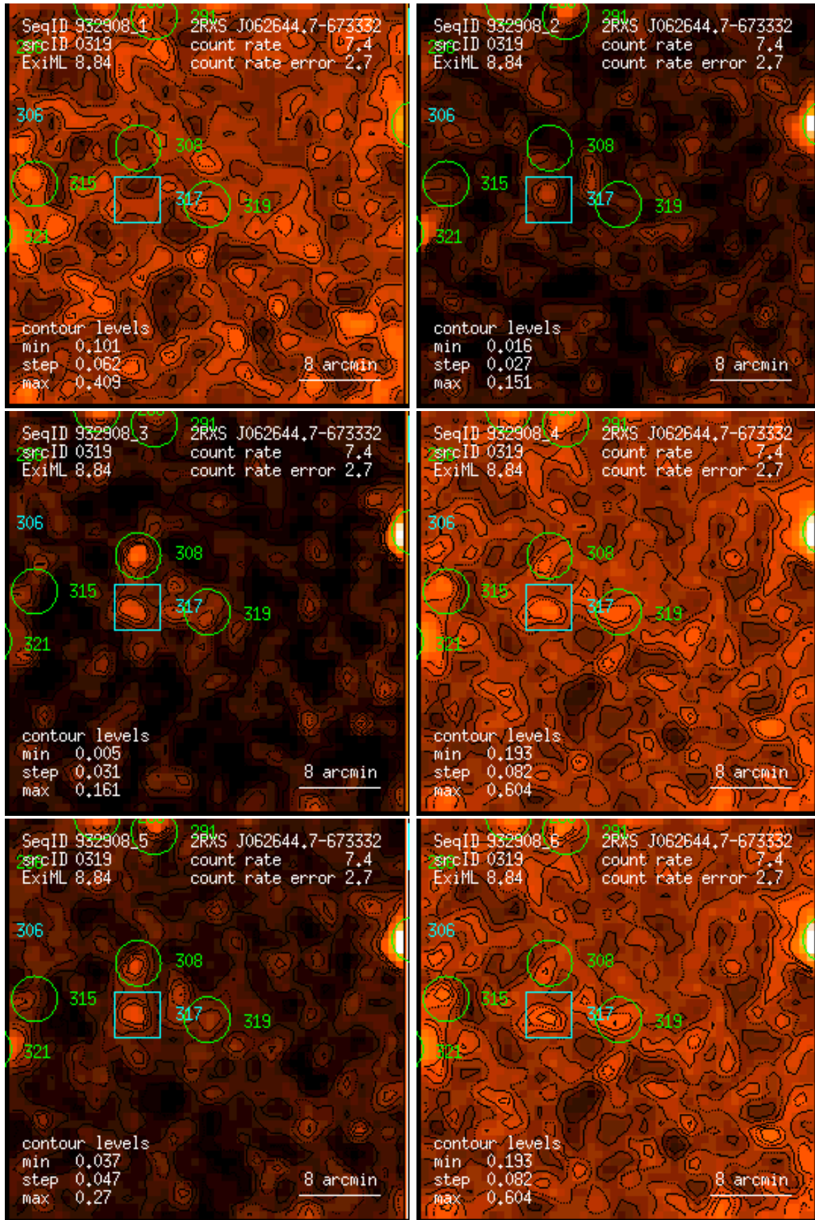
Figure 319: RASS 932908: detection 0319: band rate images, Gaussian filter: (1) PSPC channels 11 – 41, (2) 52 – 90, (3) 91 – 201, (4) 11 – 235, (5) 52 – 201, (6) 11 – 201. Broad band rates in counts/ks. Band rate contour levels in counts/ks/arcmin 2 .
