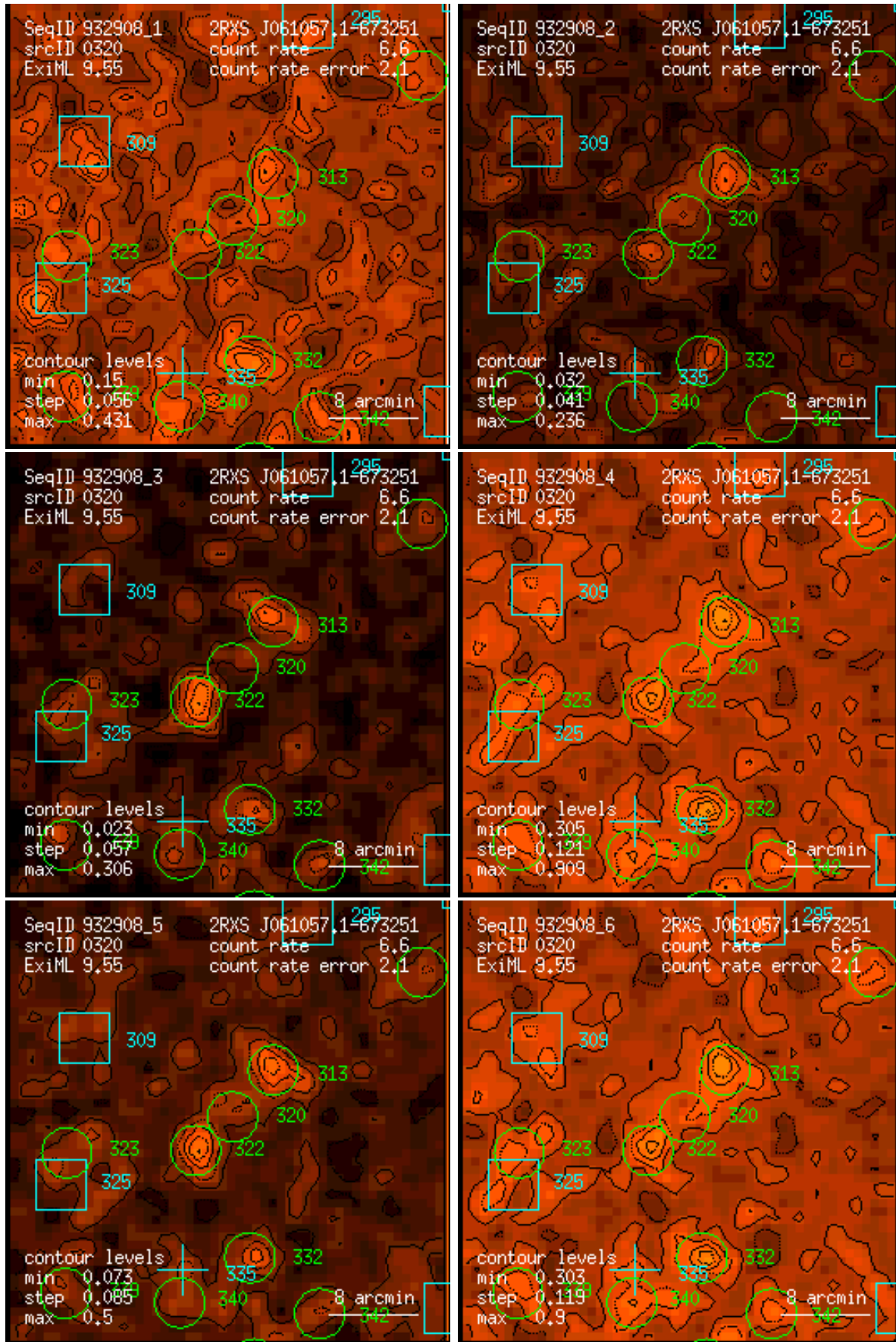
Figure 320: RASS 932908: detection 0320: band rate images, Gaussian filter: (1) PSPC channels 11 – 41, (2) 52 – 90, (3) 91 – 201, (4) 11 – 235, (5) 52 – 201, (6) 11 – 201. Broad band rates in counts/ks. Band rate contour levels in counts/ks/arcmin 2 .
