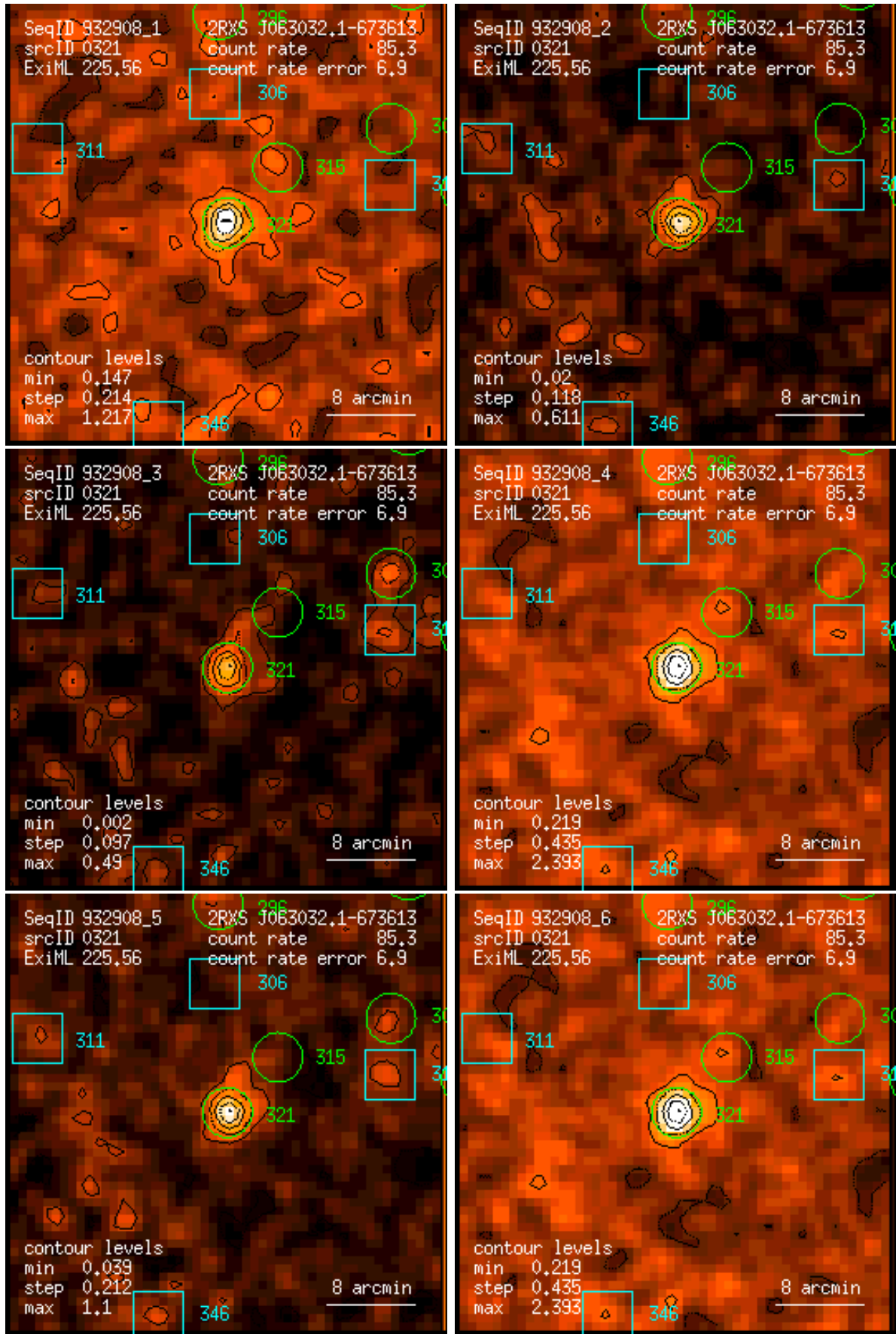
Figure 321: RASS 932908: detection 0321: band rate images, Gaussian filter: (1) PSPC channels 11 – 41, (2) 52 – 90, (3) 91 – 201, (4) 11 – 235, (5) 52 – 201, (6) 11 – 201. Broad band rates in counts/ks. Band rate contour levels in counts/ks/arcmin 2 .
