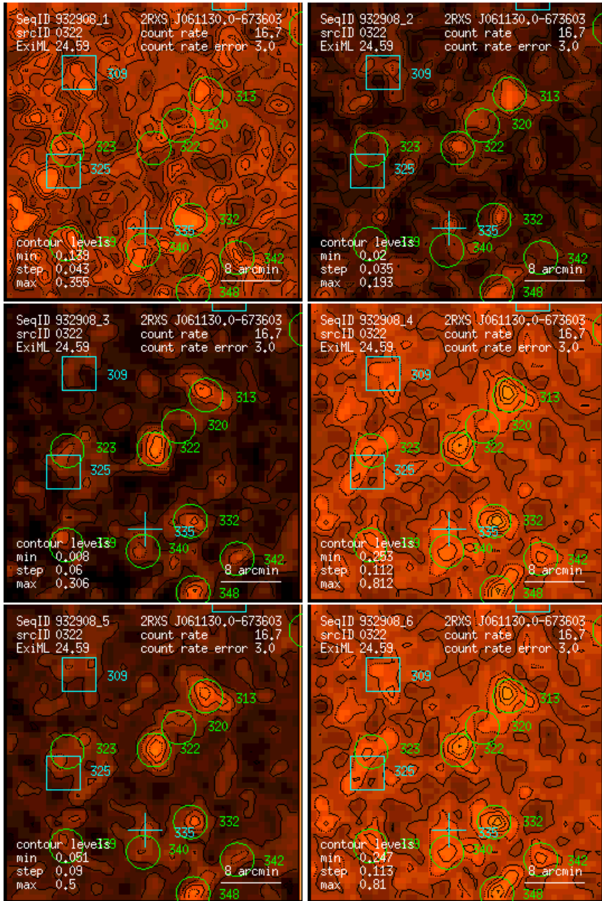
Figure 322: RASS 932908: detection 0322: band rate images, Gaussian filter: (1) PSPC channels 11 – 41, (2) 52 – 90, (3) 91 – 201, (4) 11 – 235, (5) 52 – 201, (6) 11 – 201. Broad band rates in counts/ks. Band rate contour levels in counts/ks/arcmin 2 .
