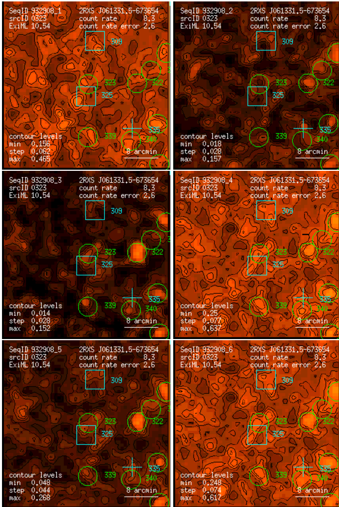
Figure 323: RASS 932908: detection 0323: band rate images, Gaussian filter: (1) PSPC channels 11 – 41, (2) 52 – 90, (3) 91 – 201, (4) 11 – 235, (5) 52 – 201, (6) 11 – 201. Broad band rates in counts/ks. Band rate contour levels in counts/ks/arcmin 2 .
