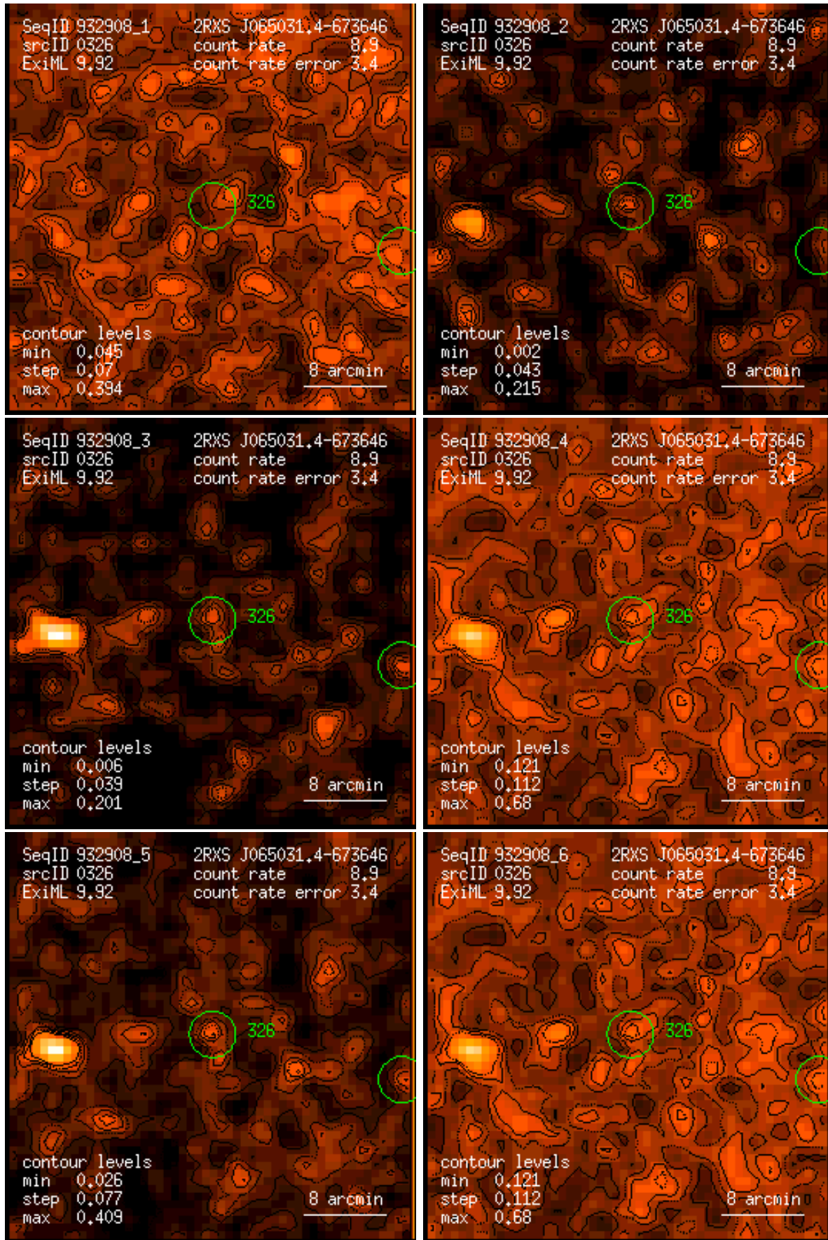
Figure 326: RASS 932908: detection 0326: band rate images, Gaussian filter: (1) PSPC channels 11 – 41, (2) 52 – 90, (3) 91 – 201, (4) 11 – 235, (5) 52 – 201, (6) 11 – 201. Broad band rates in counts/ks. Band rate contour levels in counts/ks/arcmin 2 .
