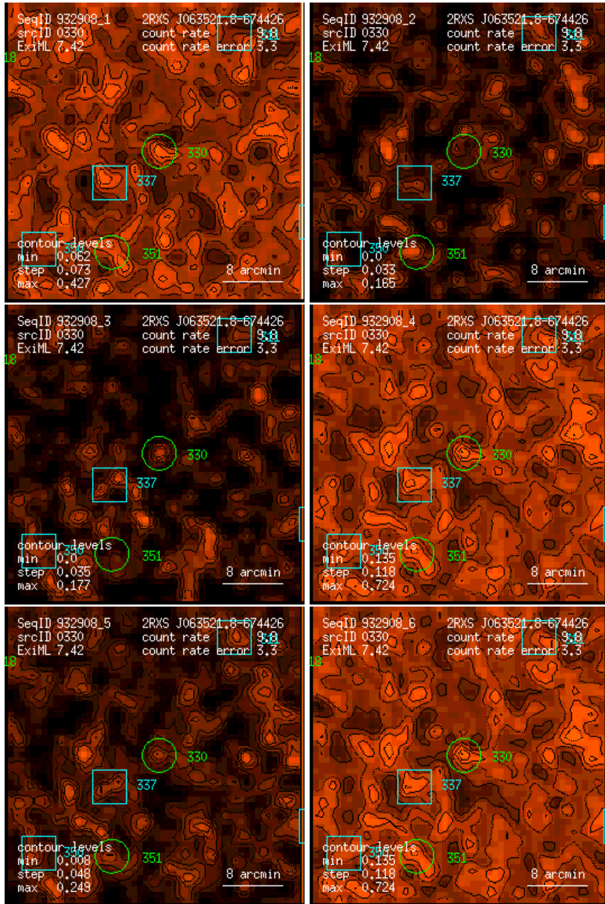
Figure 330: RASS 932908: detection 0330: band rate images, Gaussian filter: (1) PSPC channels 11 – 41, (2) 52 – 90, (3) 91 – 201, (4) 11 – 235, (5) 52 – 201, (6) 11 – 201. Broad band rates in counts/ks. Band rate contour levels in counts/ks/arcmin 2 .
