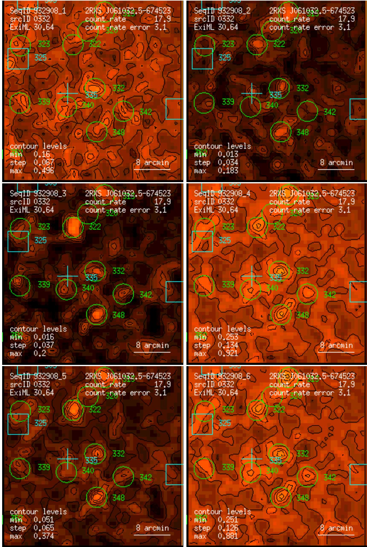
Figure 332: RASS 932908: detection 0332: band rate images, Gaussian filter: (1) PSPC channels 11 – 41, (2) 52 – 90, (3) 91 – 201, (4) 11 – 235, (5) 52 – 201, (6) 11 – 201. Broad band rates in counts/ks. Band rate contour levels in counts/ks/arcmin 2 .
