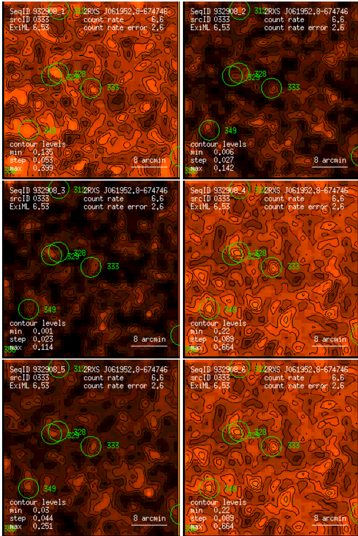
Figure 333: RASS 932908: detection 0333: band rate images, Gaussian filter: (1) PSPC channels 11 – 41, (2) 52 – 90, (3) 91 – 201, (4) 11 – 235, (5) 52 – 201, (6) 11 – 201. Broad band rates in counts/ks. Band rate contour levels in counts/ks/arcmin 2 .
