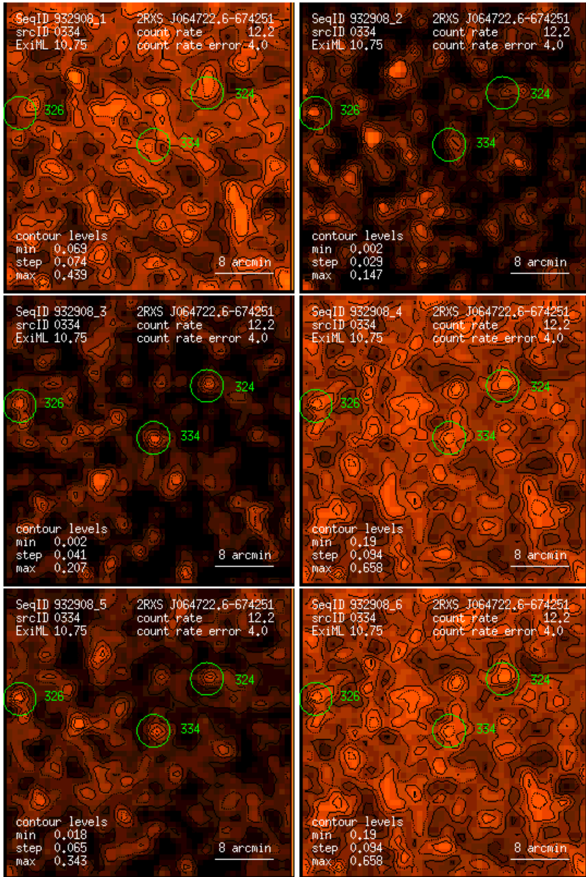
Figure 334: RASS 932908: detection 0334: band rate images, Gaussian filter: (1) PSPC channels 11 – 41, (2) 52 – 90, (3) 91 – 201, (4) 11 – 235, (5) 52 – 201, (6) 11 – 201. Broad band rates in counts/ks. Band rate contour levels in counts/ks/arcmin 2 .
