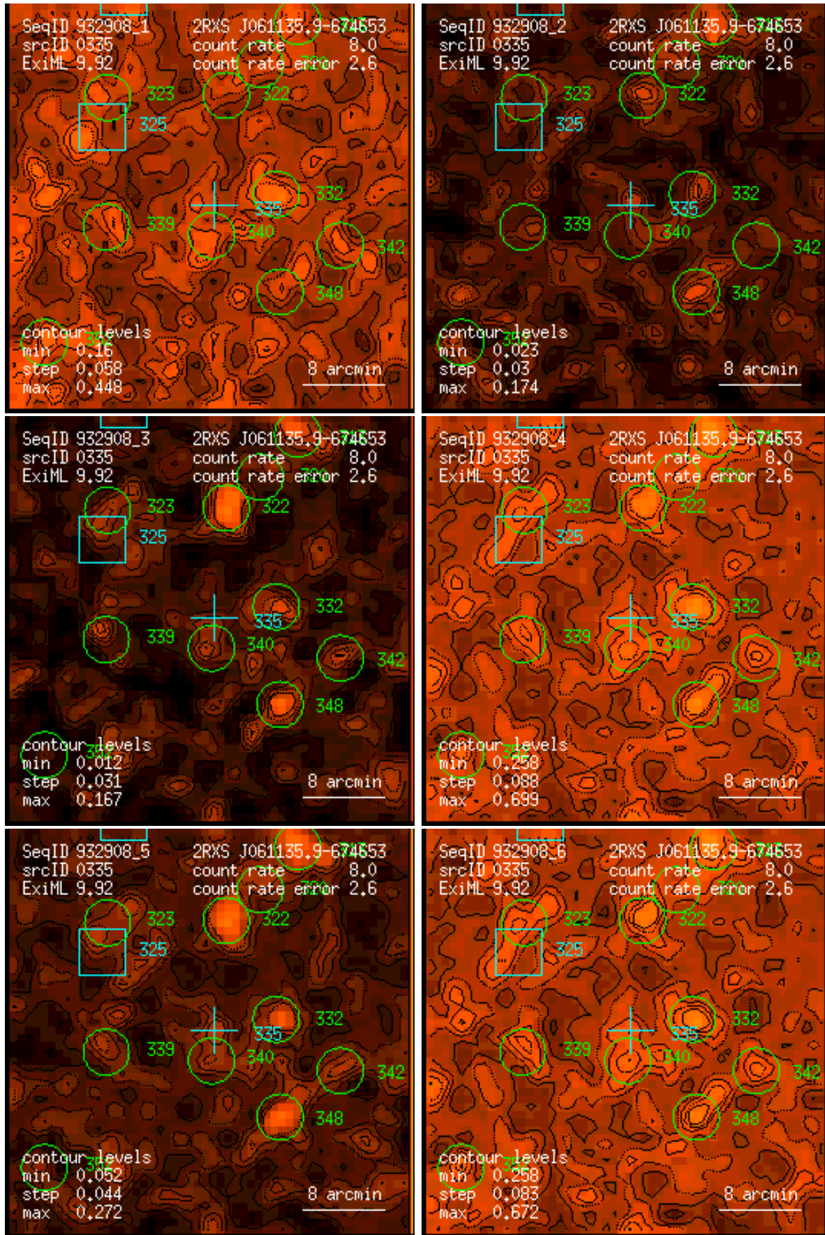
Figure 335: RASS 932908: detection 0335: band rate images, Gaussian filter: (1) PSPC channels 11 – 41, (2) 52 – 90, (3) 91 – 201, (4) 11 – 235, (5) 52 – 201, (6) 11 – 201. Broad band rates in counts/ks. Band rate contour levels in counts/ks/arcmin 2 .
