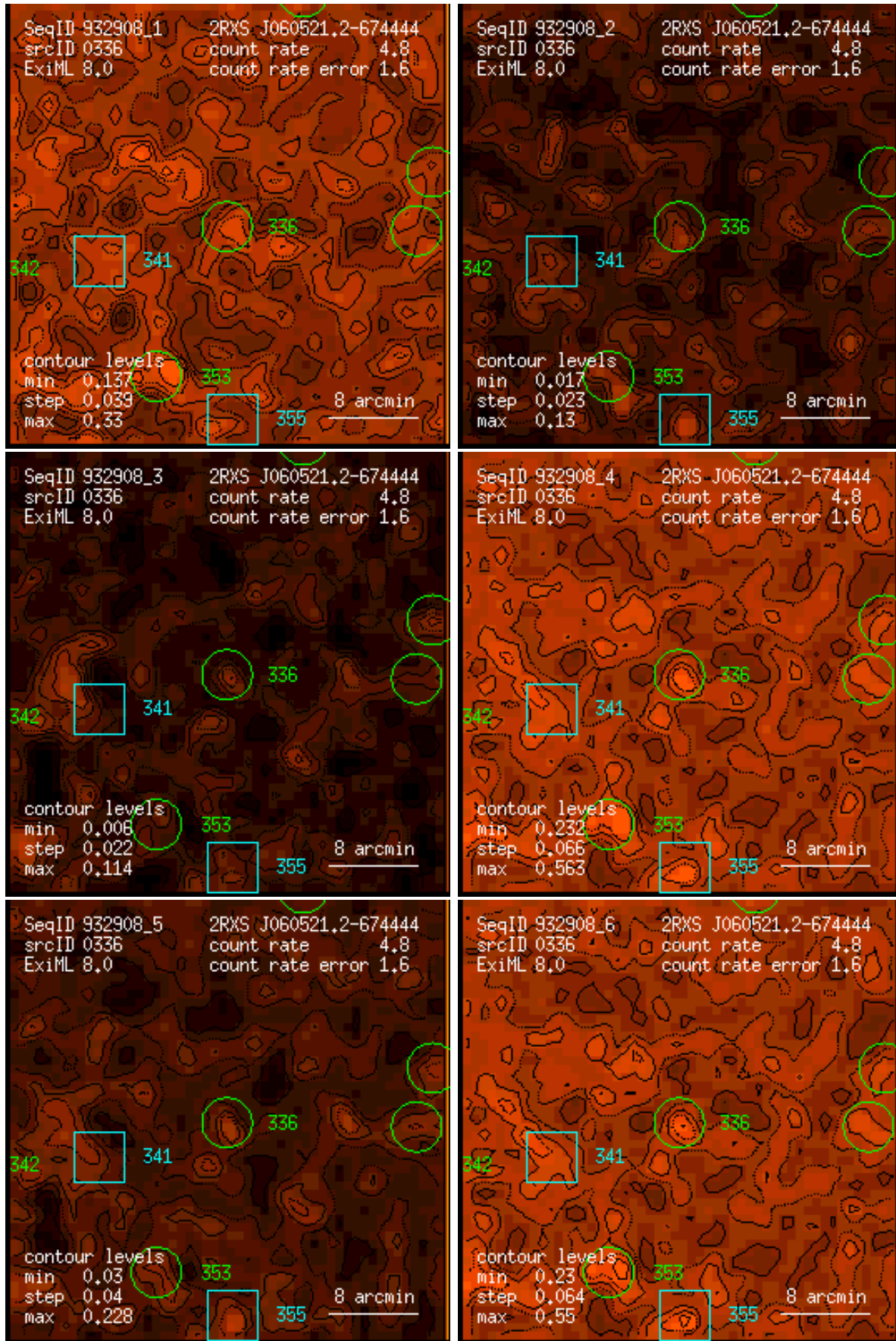
Figure 336: RASS 932908: detection 0336: band rate images, Gaussian filter: (1) PSPC channels 11 – 41, (2) 52 – 90, (3) 91 – 201, (4) 11 – 235, (5) 52 – 201, (6) 11 – 201. Broad band rates in counts/ks. Band rate contour levels in counts/ks/arcmin 2 .
