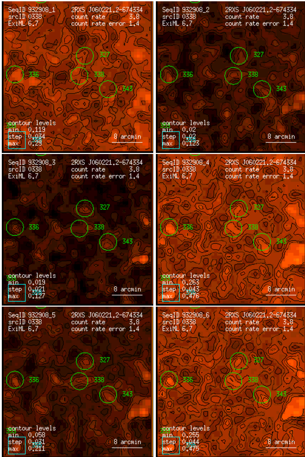
Figure 338: RASS 932908: detection 0338: band rate images, Gaussian filter: (1) PSPC channels 11 – 41, (2) 52 – 90, (3) 91 – 201, (4) 11 – 235, (5) 52 – 201, (6) 11 – 201. Broad band rates in counts/ks. Band rate contour levels in counts/ks/arcmin 2 .
