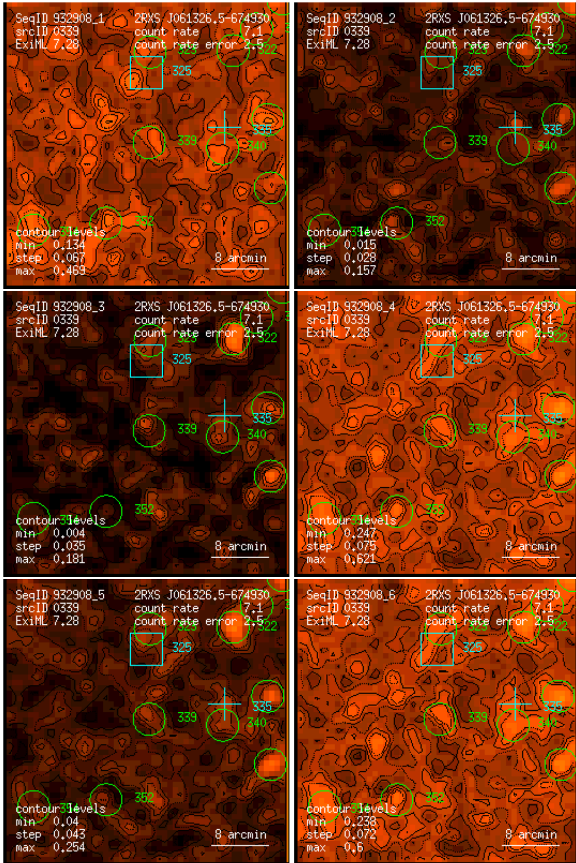
Figure 339: RASS 932908: detection 0339: band rate images, Gaussian filter: (1) PSPC channels 11 – 41, (2) 52 – 90, (3) 91 – 201, (4) 11 – 235, (5) 52 – 201, (6) 11 – 201. Broad band rates in counts/ks. Band rate contour levels in counts/ks/arcmin 2 .
