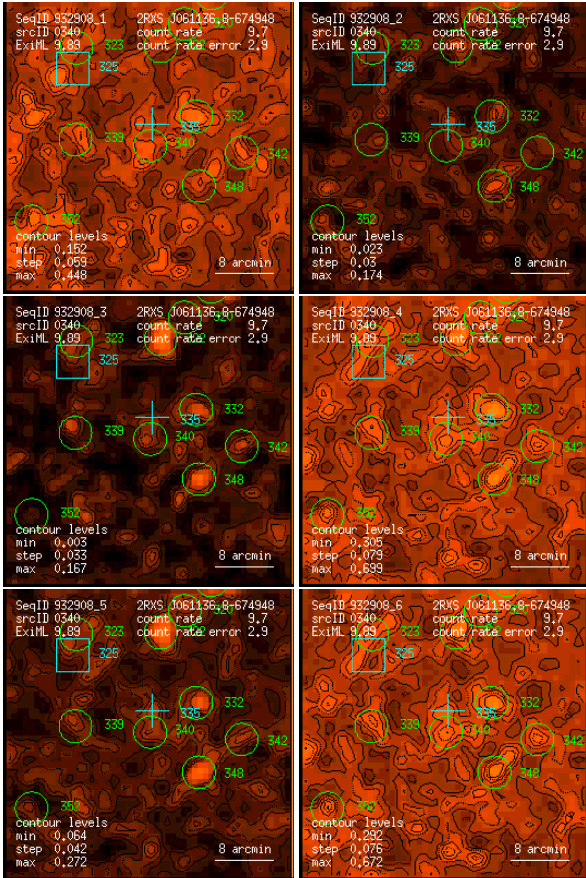
Figure 340: RASS 932908: detection 0340: band rate images, Gaussian filter: (1) PSPC channels 11 – 41, (2) 52 – 90, (3) 91 – 201, (4) 11 – 235, (5) 52 – 201, (6) 11 – 201. Broad band rates in counts/ks. Band rate contour levels in counts/ks/arcmin 2 .
