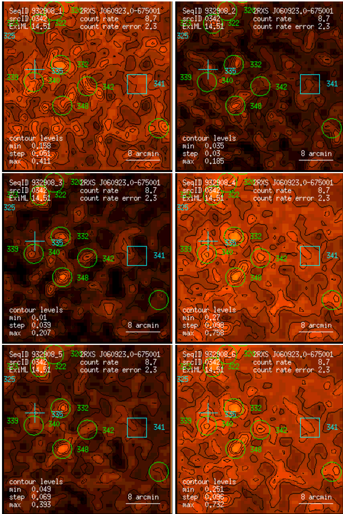
Figure 342: RASS 932908: detection 0342: band rate images, Gaussian filter: (1) PSPC channels 11 – 41, (2) 52 – 90, (3) 91 – 201, (4) 11 – 235, (5) 52 – 201, (6) 11 – 201. Broad band rates in counts/ks. Band rate contour levels in counts/ks/arcmin 2 .
