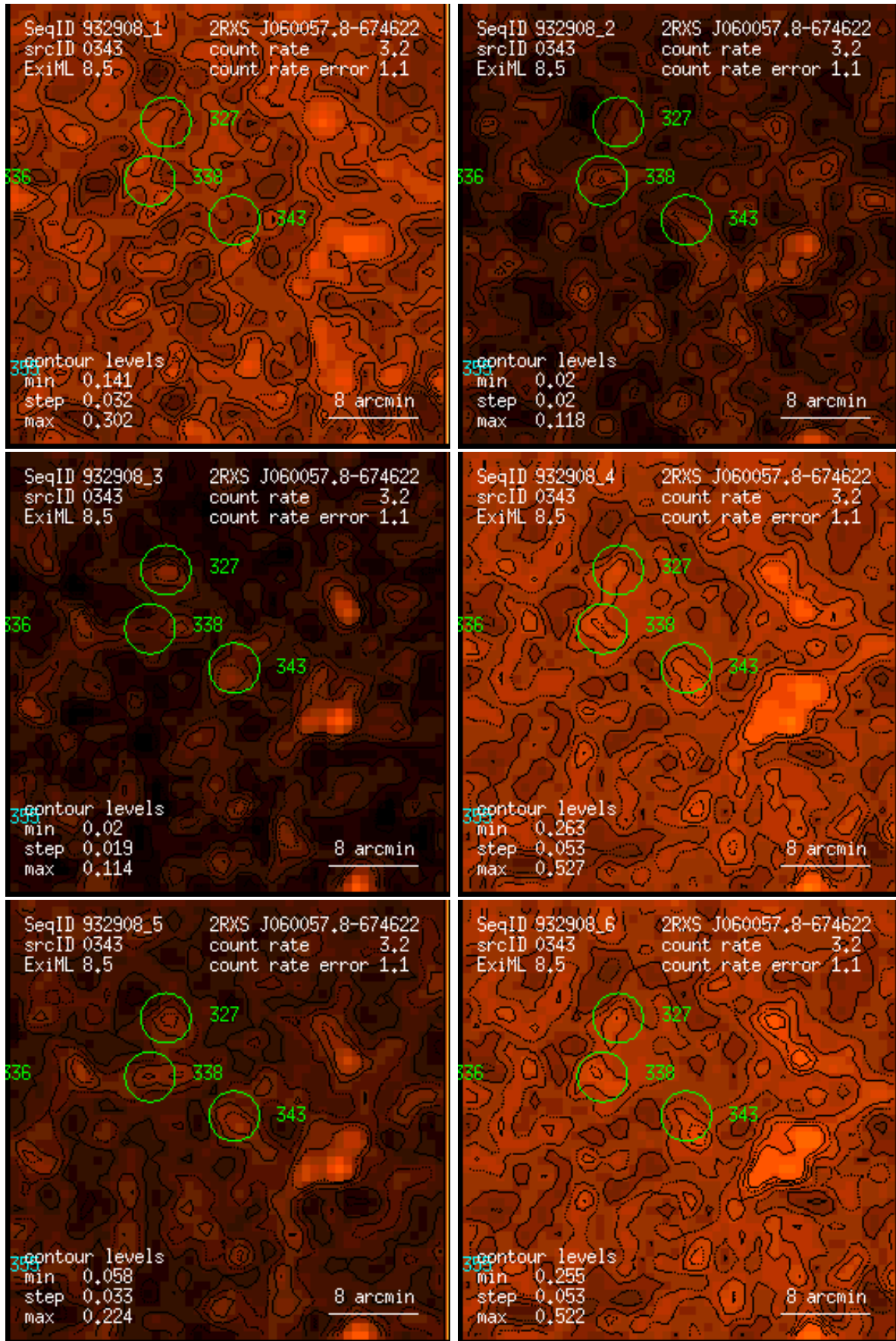
Figure 343: RASS 932908: detection 0343: band rate images, Gaussian filter: (1) PSPC channels 11 – 41, (2) 52 – 90, (3) 91 – 201, (4) 11 – 235, (5) 52 – 201, (6) 11 – 201. Broad band rates in counts/ks. Band rate contour levels in counts/ks/arcmin 2 .
