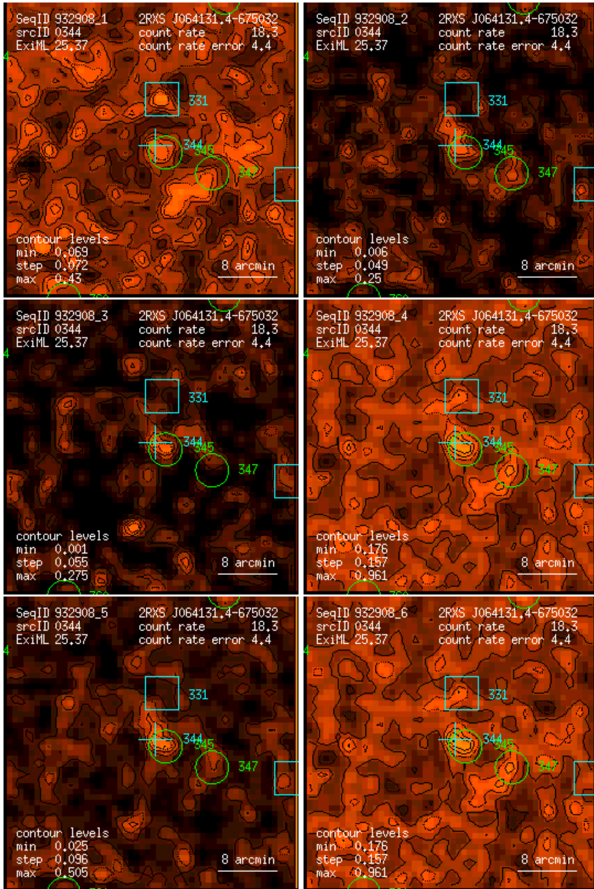
Figure 344: RASS 932908: detection 0344: band rate images, Gaussian filter: (1) PSPC channels 11 – 41, (2) 52 – 90, (3) 91 – 201, (4) 11 – 235, (5) 52 – 201, (6) 11 – 201. Broad band rates in counts/ks. Band rate contour levels in counts/ks/arcmin 2 .
