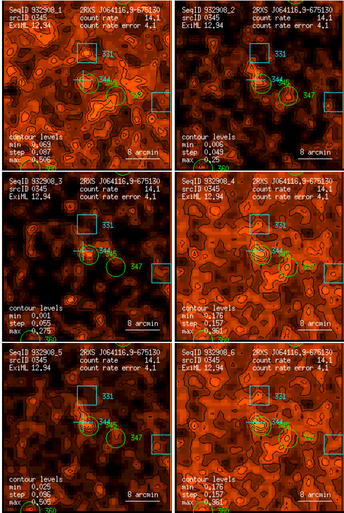
Figure 345: RASS 932908: detection 0345: band rate images, Gaussian filter: (1) PSPC channels 11 – 41, (2) 52 – 90, (3) 91 – 201, (4) 11 – 235, (5) 52 – 201, (6) 11 – 201. Broad band rates in counts/ks. Band rate contour levels in counts/ks/arcmin 2 .
