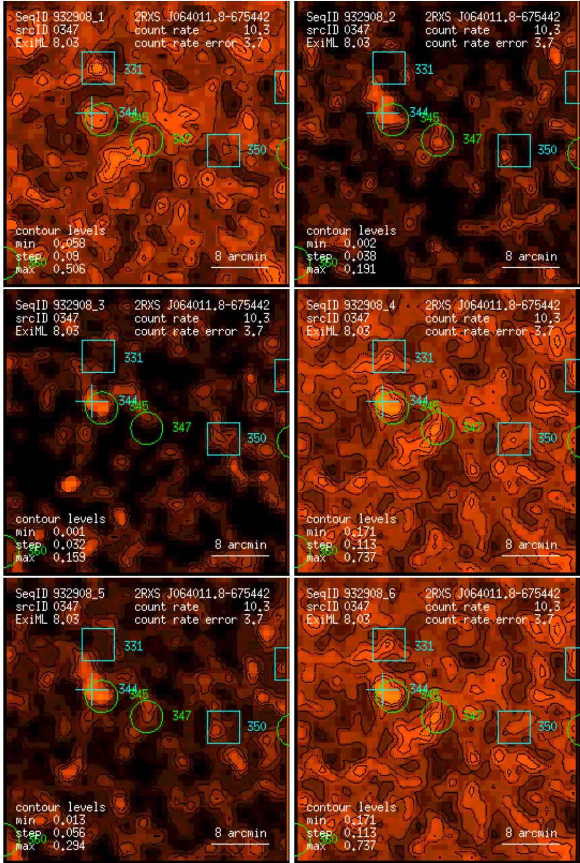
Figure 347: RASS 932908: detection 0347: band rate images, Gaussian filter: (1) PSPC channels 11 – 41, (2) 52 – 90, (3) 91 – 201, (4) 11 – 235, (5) 52 – 201, (6) 11 – 201. Broad band rates in counts/ks. Band rate contour levels in counts/ks/arcmin 2 .
