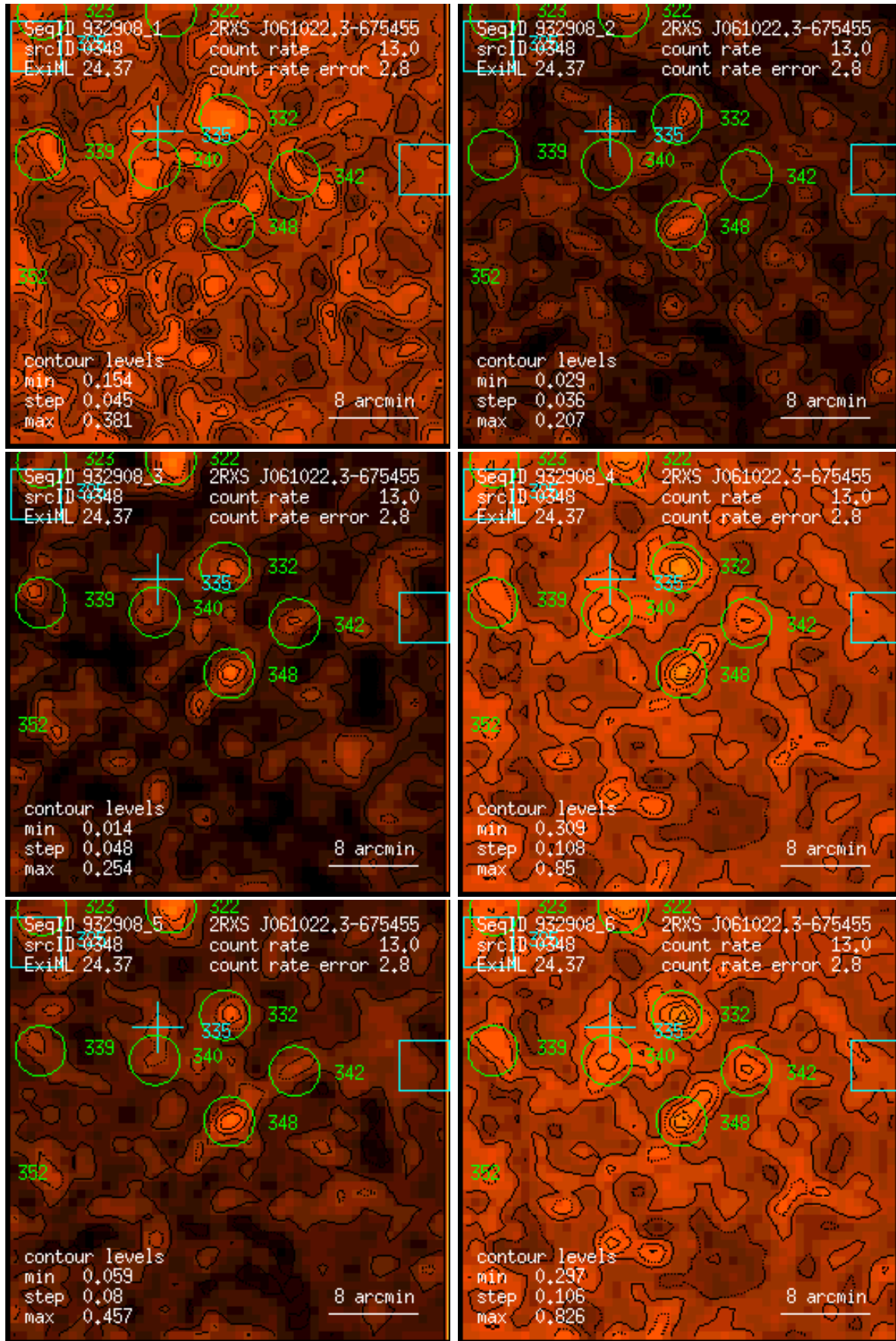
Figure 348: RASS 932908: detection 0348: band rate images, Gaussian filter: (1) PSPC channels 11 – 41, (2) 52 – 90, (3) 91 – 201, (4) 11 – 235, (5) 52 – 201, (6) 11 – 201. Broad band rates in counts/ks. Band rate contour levels in counts/ks/arcmin 2 .
