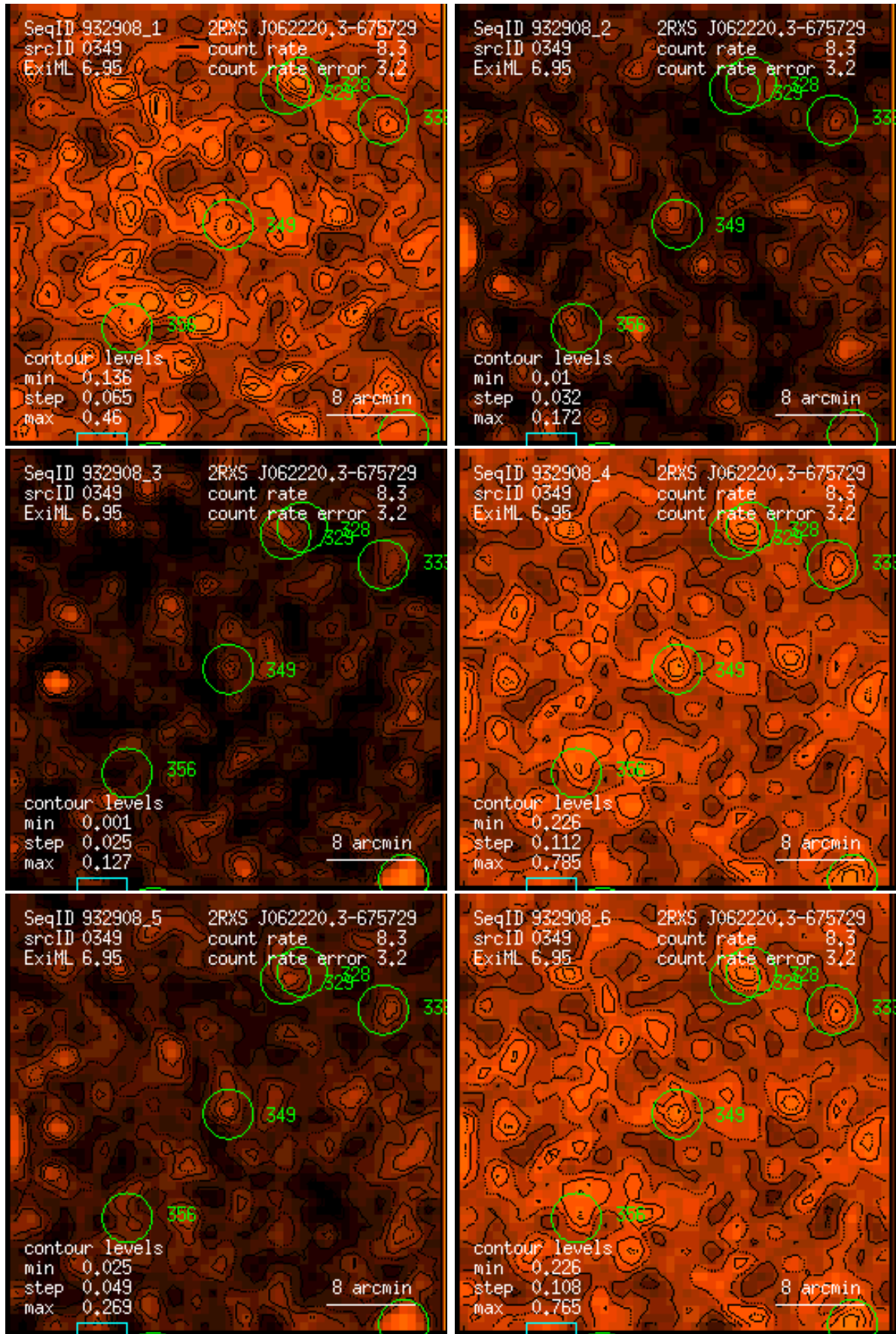
Figure 349: RASS 932908: detection 0349: band rate images, Gaussian filter: (1) PSPC channels 11 – 41, (2) 52 – 90, (3) 91 – 201, (4) 11 – 235, (5) 52 – 201, (6) 11 – 201. Broad band rates in counts/ks. Band rate contour levels in counts/ks/arcmin 2 .
