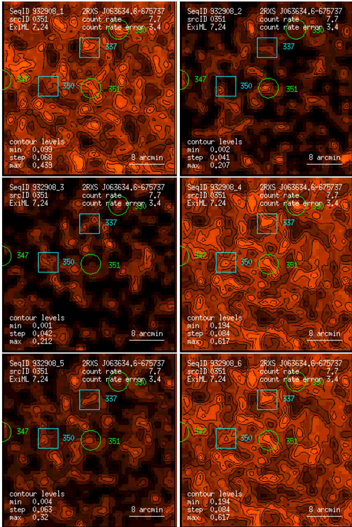
Figure 351: RASS 932908: detection 0351: band rate images, Gaussian filter: (1) PSPC channels 11 – 41, (2) 52 – 90, (3) 91 – 201, (4) 11 – 235, (5) 52 – 201, (6) 11 – 201. Broad band rates in counts/ks. Band rate contour levels in counts/ks/arcmin 2 .
