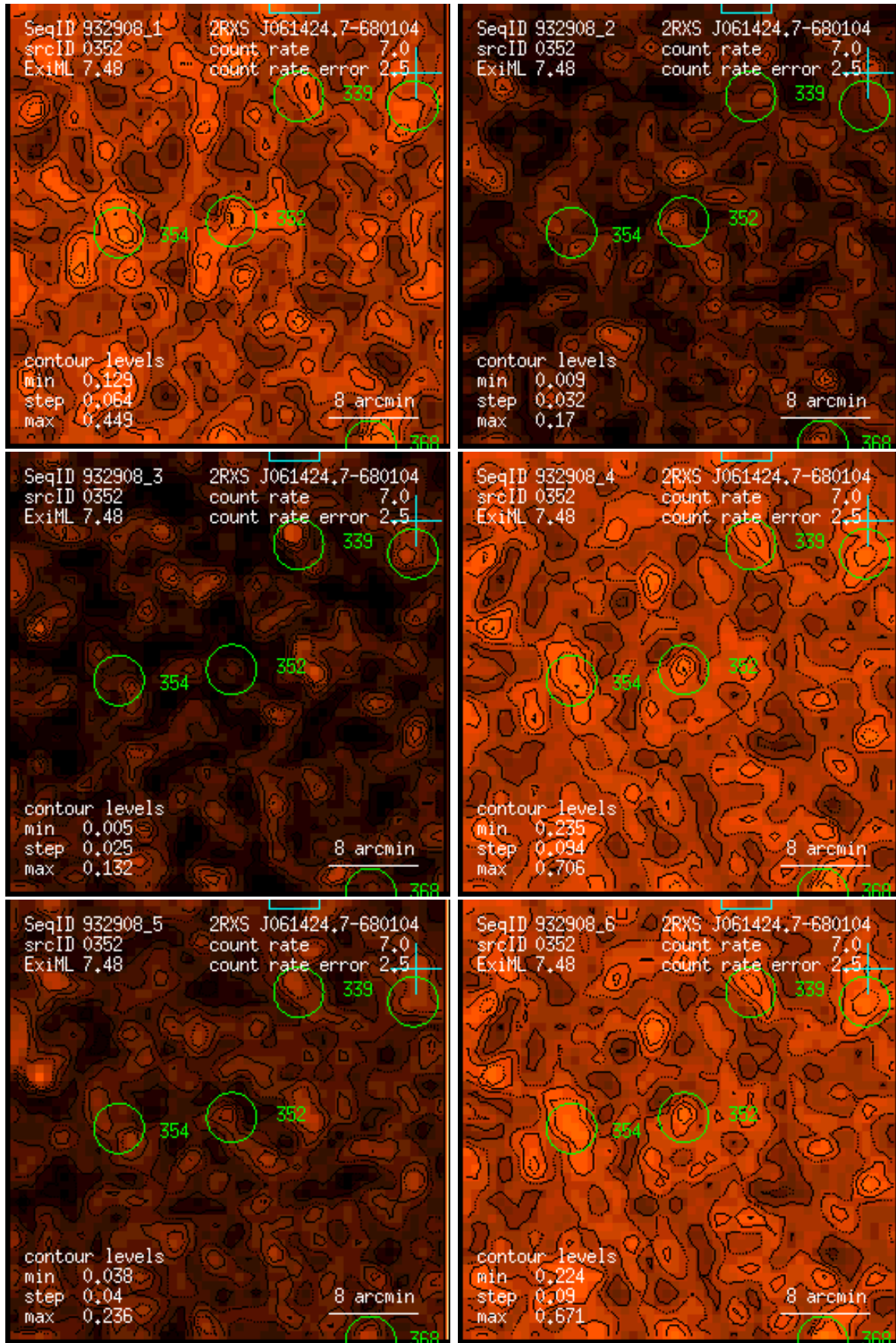
Figure 352: RASS 932908: detection 0352: band rate images, Gaussian filter: (1) PSPC channels 11 – 41, (2) 52 – 90, (3) 91 – 201, (4) 11 – 235, (5) 52 – 201, (6) 11 – 201. Broad band rates in counts/ks. Band rate contour levels in counts/ks/arcmin 2 .
